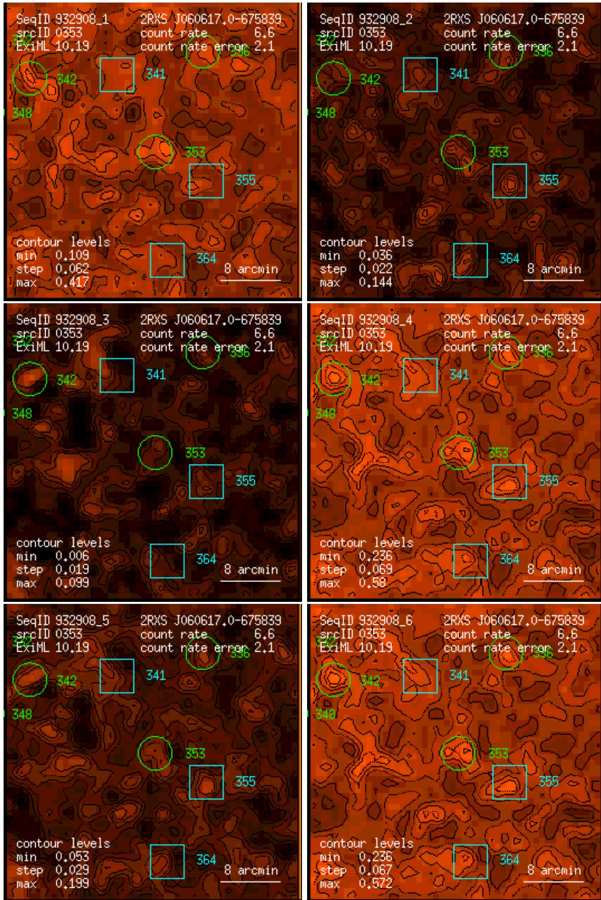
Figure 353: RASS 932908: detection 0353: band rate images, Gaussian filter: (1) PSPC channels 11 – 41, (2) 52 – 90, (3) 91 – 201, (4) 11 – 235, (5) 52 – 201, (6) 11 – 201. Broad band rates in counts/ks. Band rate contour levels in counts/ks/arcmin 2 .
