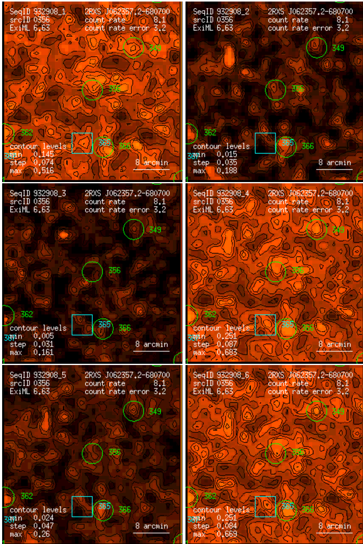
Figure 356: RASS 932908: detection 0356: band rate images, Gaussian filter: (1) PSPC channels 11 – 41, (2) 52 – 90, (3) 91 – 201, (4) 11 – 235, (5) 52 – 201, (6) 11 – 201. Broad band rates in counts/ks. Band rate contour levels in counts/ks/arcmin 2 .
