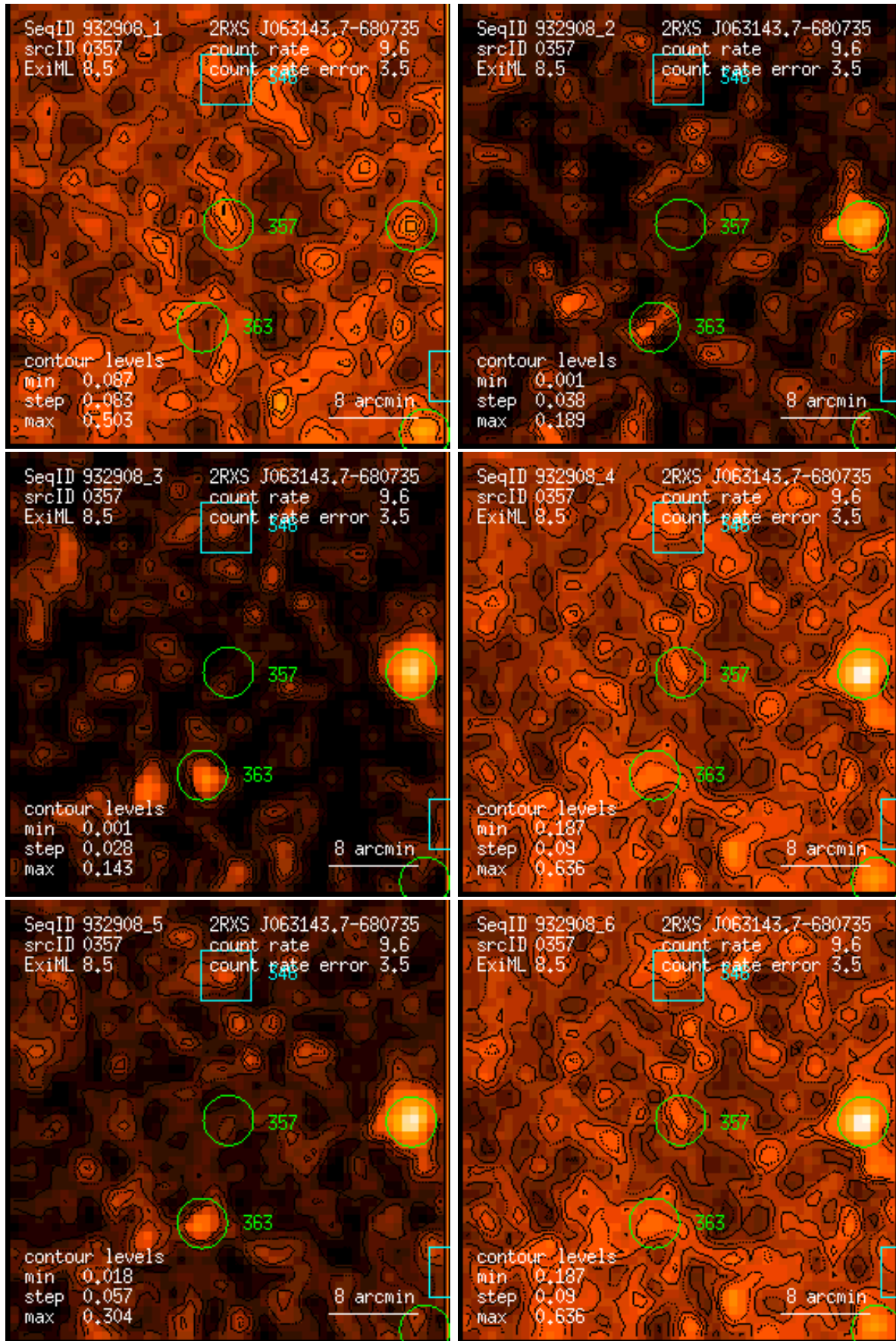
Figure 357: RASS 932908: detection 0357: band rate images, Gaussian filter: (1) PSPC channels 11 – 41, (2) 52 – 90, (3) 91 – 201, (4) 11 – 235, (5) 52 – 201, (6) 11 – 201. Broad band rates in counts/ks. Band rate contour levels in counts/ks/arcmin 2 .
