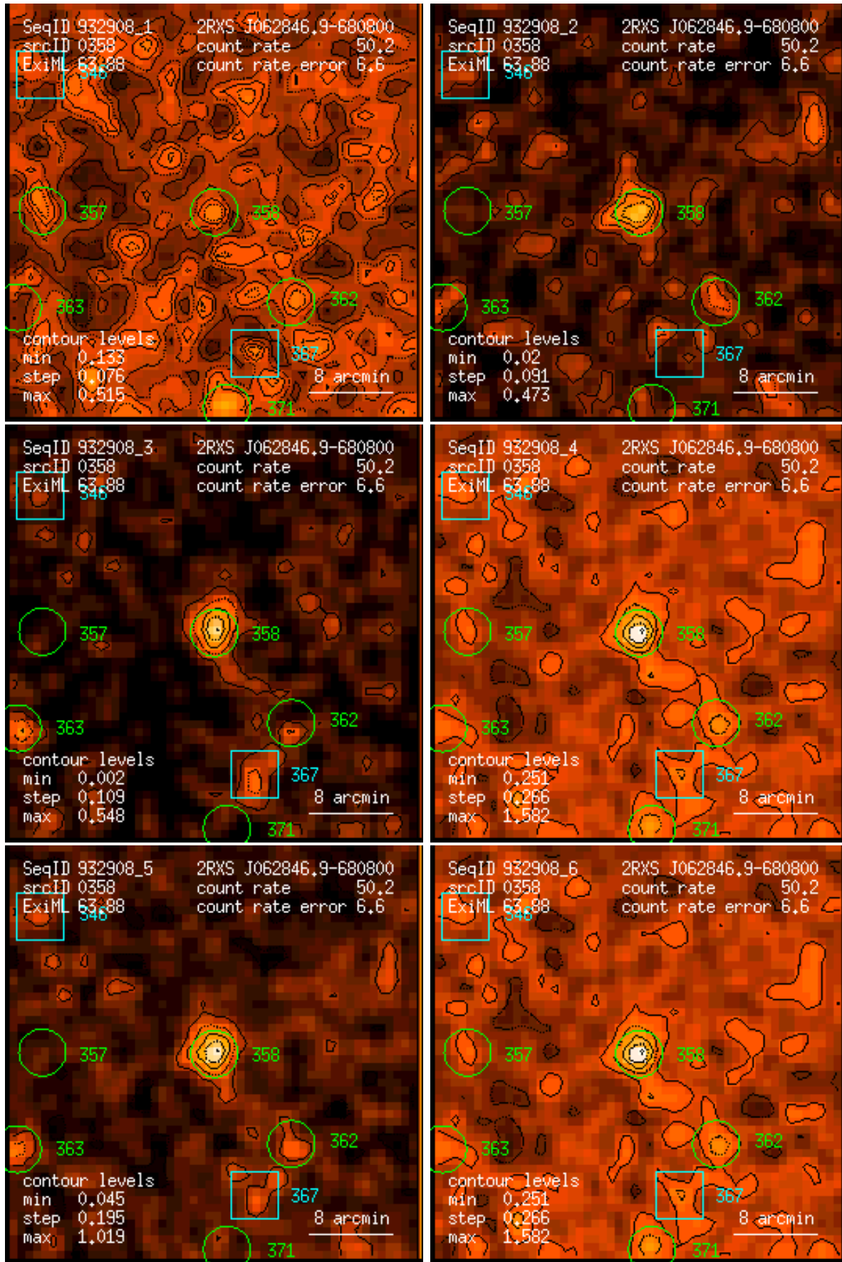
Figure 358: RASS 932908: detection 0358: band rate images, Gaussian filter: (1) PSPC channels 11 – 41, (2) 52 – 90, (3) 91 – 201, (4) 11 – 235, (5) 52 – 201, (6) 11 – 201. Broad band rates in counts/ks. Band rate contour levels in counts/ks/arcmin 2 .
