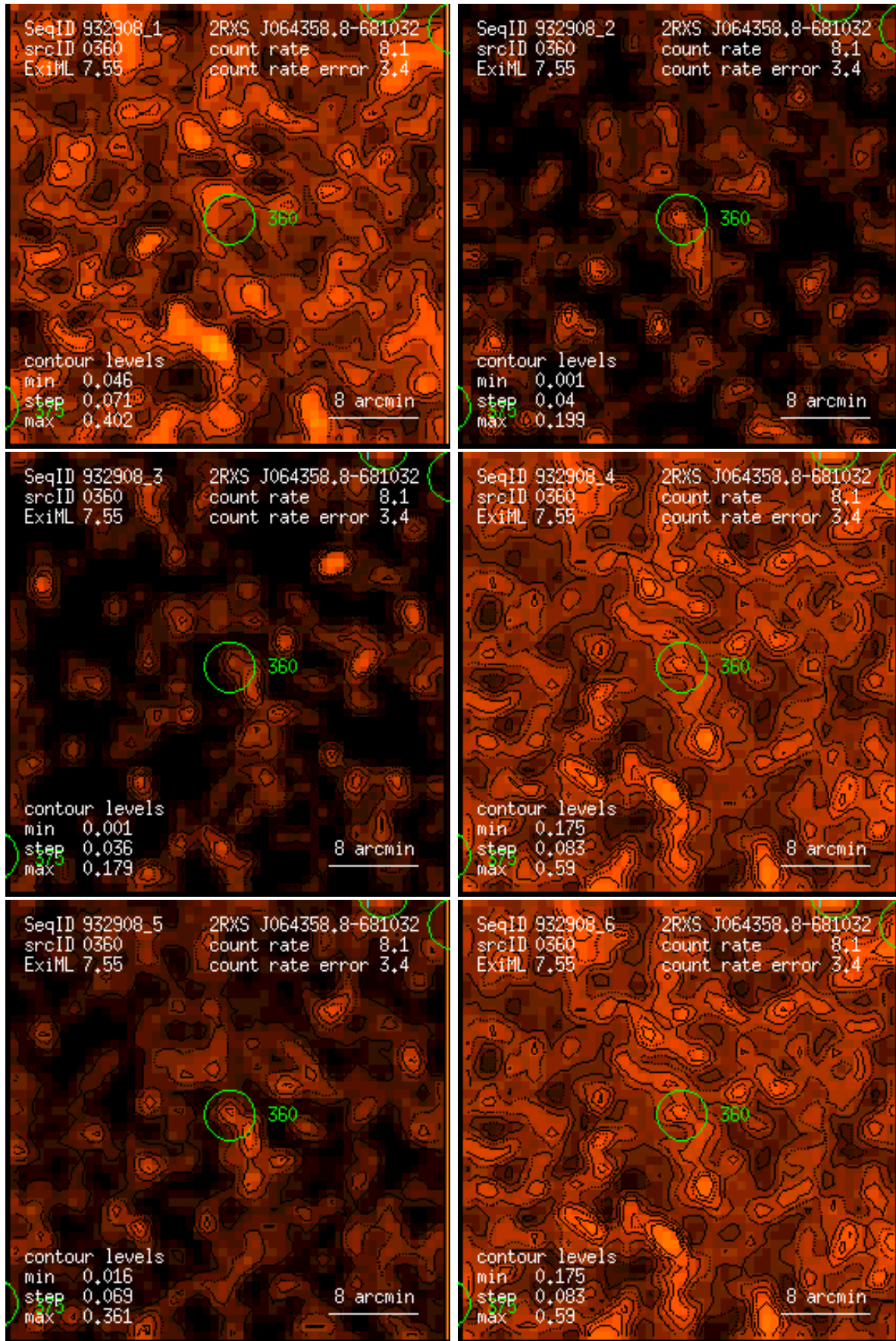
Figure 360: RASS 932908: detection 0360: band rate images, Gaussian filter: (1) PSPC channels 11 – 41, (2) 52 – 90, (3) 91 – 201, (4) 11 – 235, (5) 52 – 201, (6) 11 – 201. Broad band rates in counts/ks. Band rate contour levels in counts/ks/arcmin 2 .
