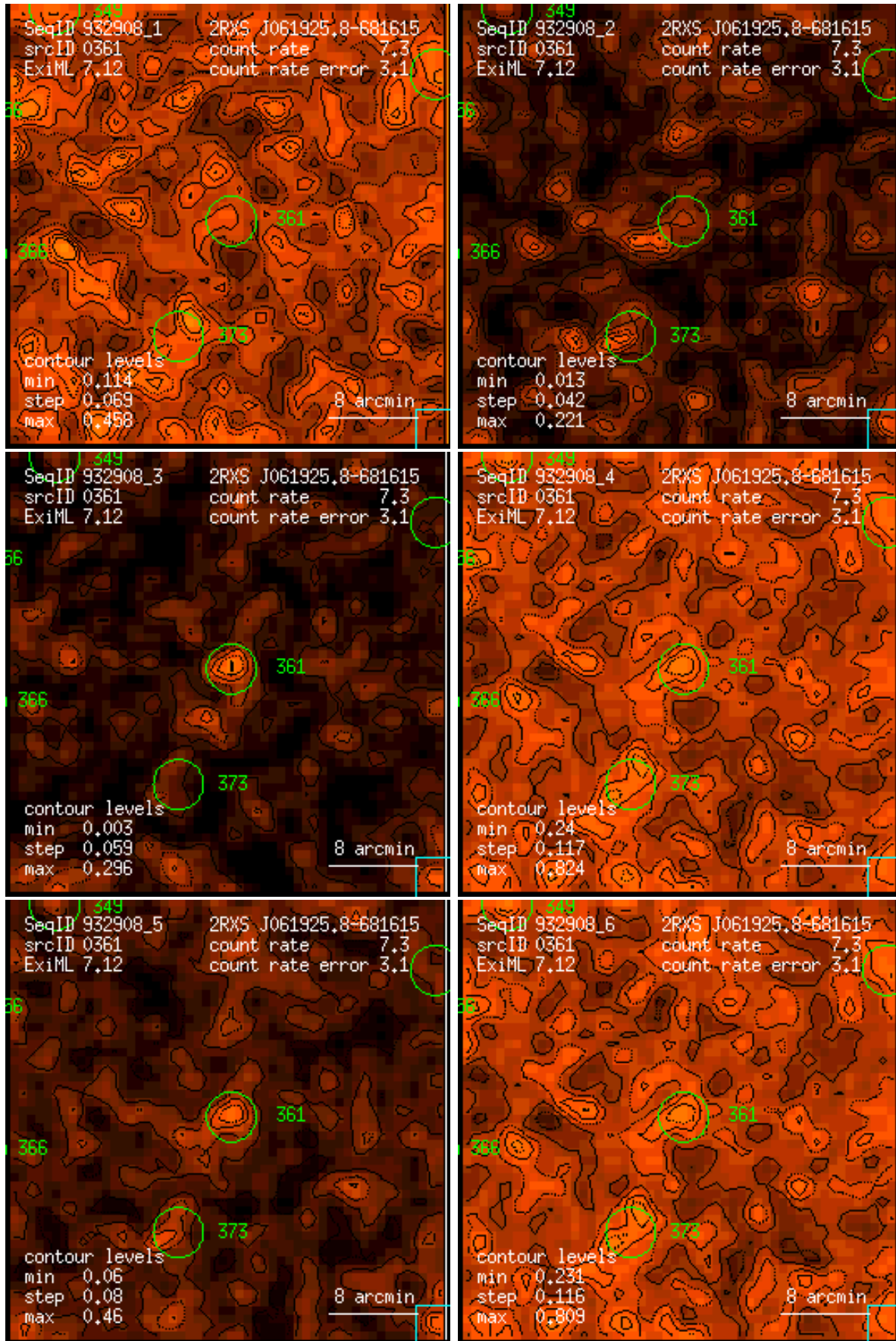
Figure 361: RASS 932908: detection 0361: band rate images, Gaussian filter: (1) PSPC channels 11 – 41, (2) 52 – 90, (3) 91 – 201, (4) 11 – 235, (5) 52 – 201, (6) 11 – 201. Broad band rates in counts/ks. Band rate contour levels in counts/ks/arcmin 2 .
