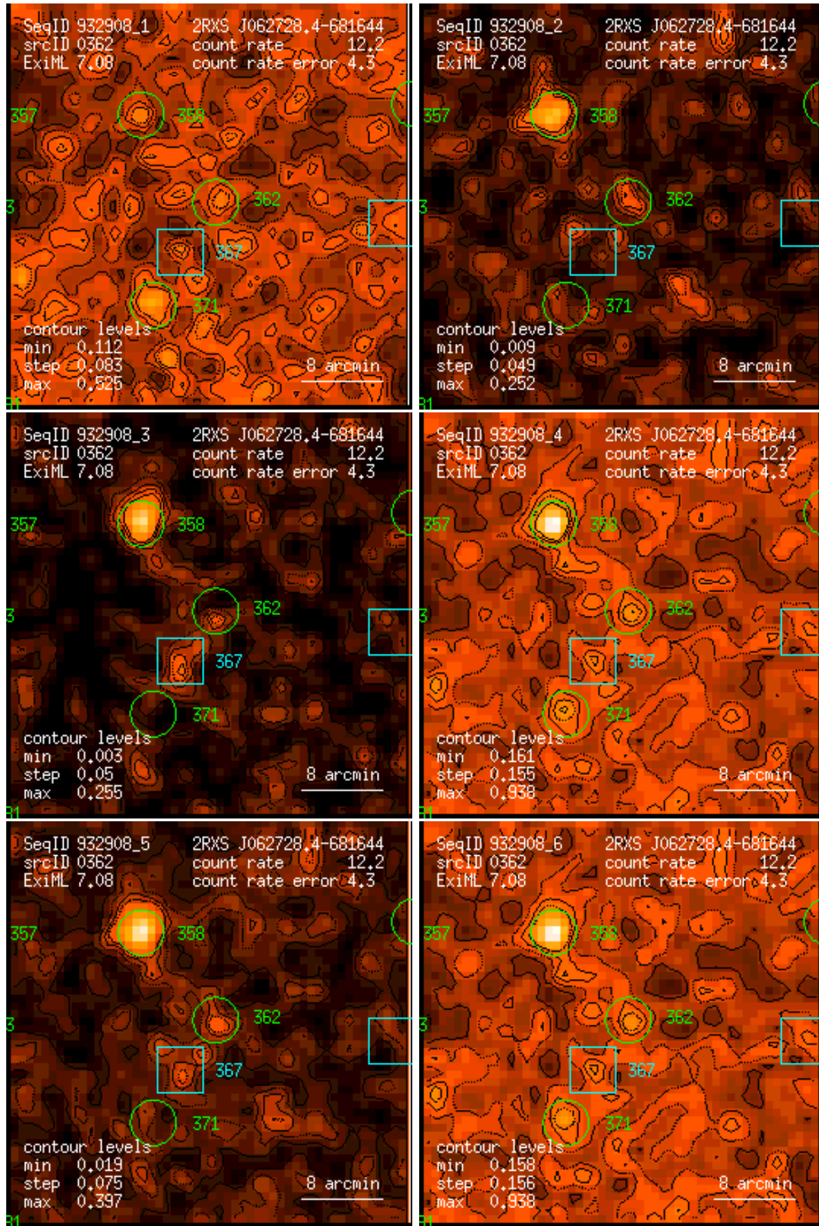
Figure 362: RASS 932908: detection 0362: band rate images, Gaussian filter: (1) PSPC channels 11 – 41, (2) 52 – 90, (3) 91 – 201, (4) 11 – 235, (5) 52 – 201, (6) 11 – 201. Broad band rates in counts/ks. Band rate contour levels in counts/ks/arcmin 2 .
