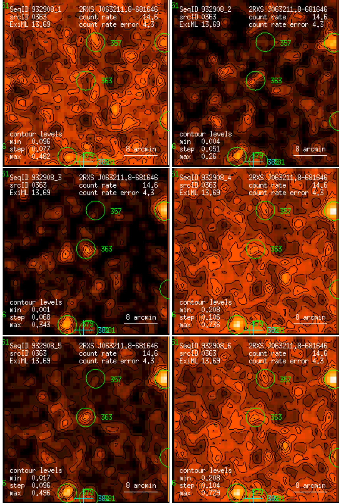
Figure 363: RASS 932908: detection 0363: band rate images, Gaussian filter: (1) PSPC channels 11 – 41, (2) 52 – 90, (3) 91 – 201, (4) 11 – 235, (5) 52 – 201, (6) 11 – 201. Broad band rates in counts/ks. Band rate contour levels in counts/ks/arcmin 2 .
