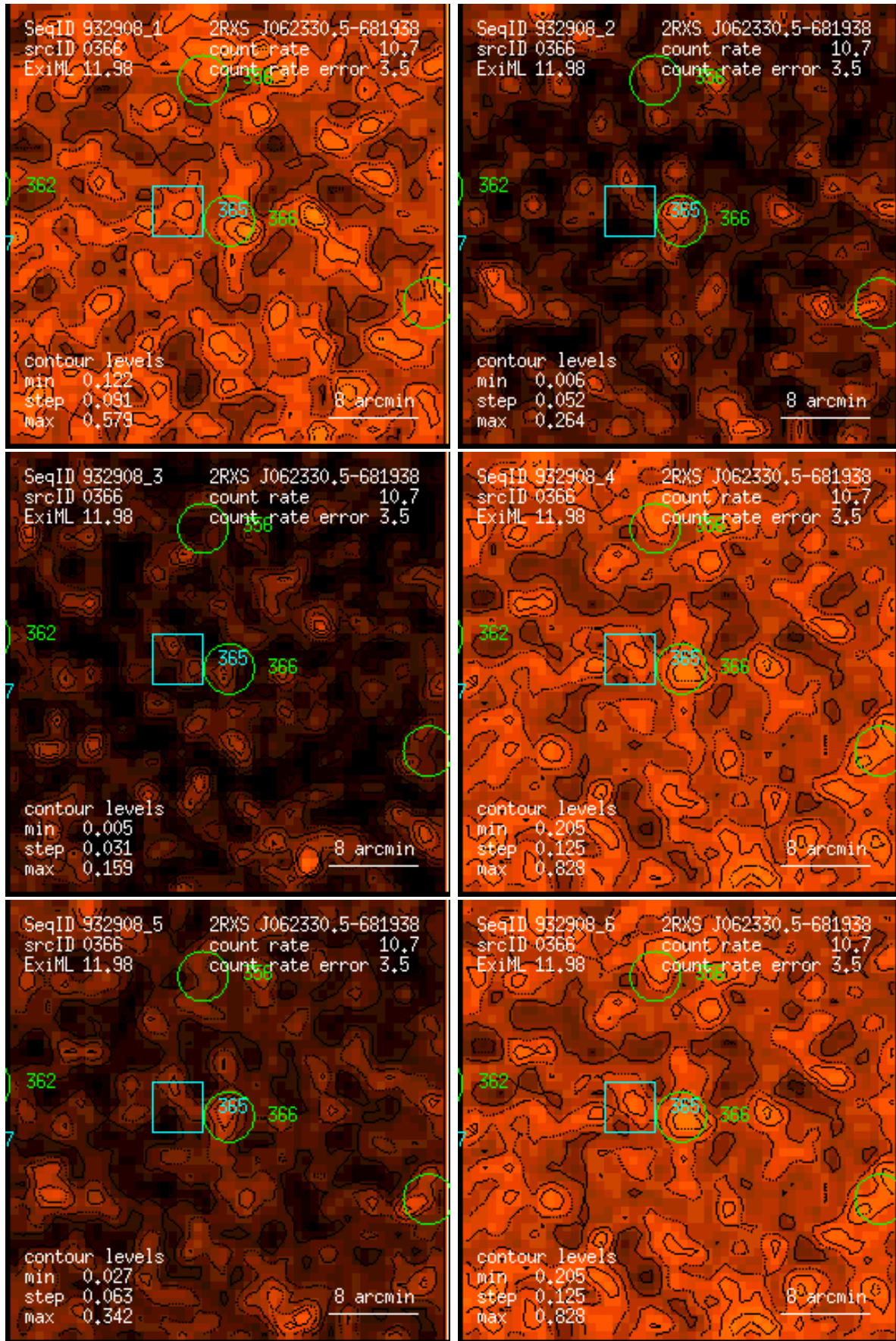
Figure 366: RASS 932908: detection 0366: band rate images, Gaussian filter: (1) PSPC channels 11 – 41, (2) 52 – 90, (3) 91 – 201, (4) 11 – 235, (5) 52 – 201, (6) 11 – 201. Broad band rates in counts/ks. Band rate contour levels in counts/ks/arcmin 2 .
