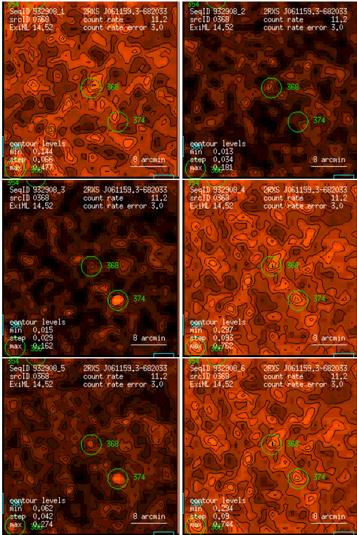
Figure 368: RASS 932908: detection 0368: band rate images, Gaussian filter: (1) PSPC channels 11 – 41, (2) 52 – 90, (3) 91 – 201, (4) 11 – 235, (5) 52 – 201, (6) 11 – 201. Broad band rates in counts/ks. Band rate contour levels in counts/ks/arcmin 2 .
