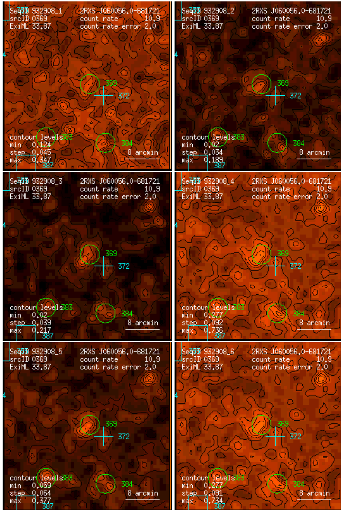
Figure 369: RASS 932908: detection 0369: band rate images, Gaussian filter: (1) PSPC channels 11 – 41, (2) 52 – 90, (3) 91 – 201, (4) 11 – 235, (5) 52 – 201, (6) 11 – 201. Broad band rates in counts/ks. Band rate contour levels in counts/ks/arcmin 2 .
