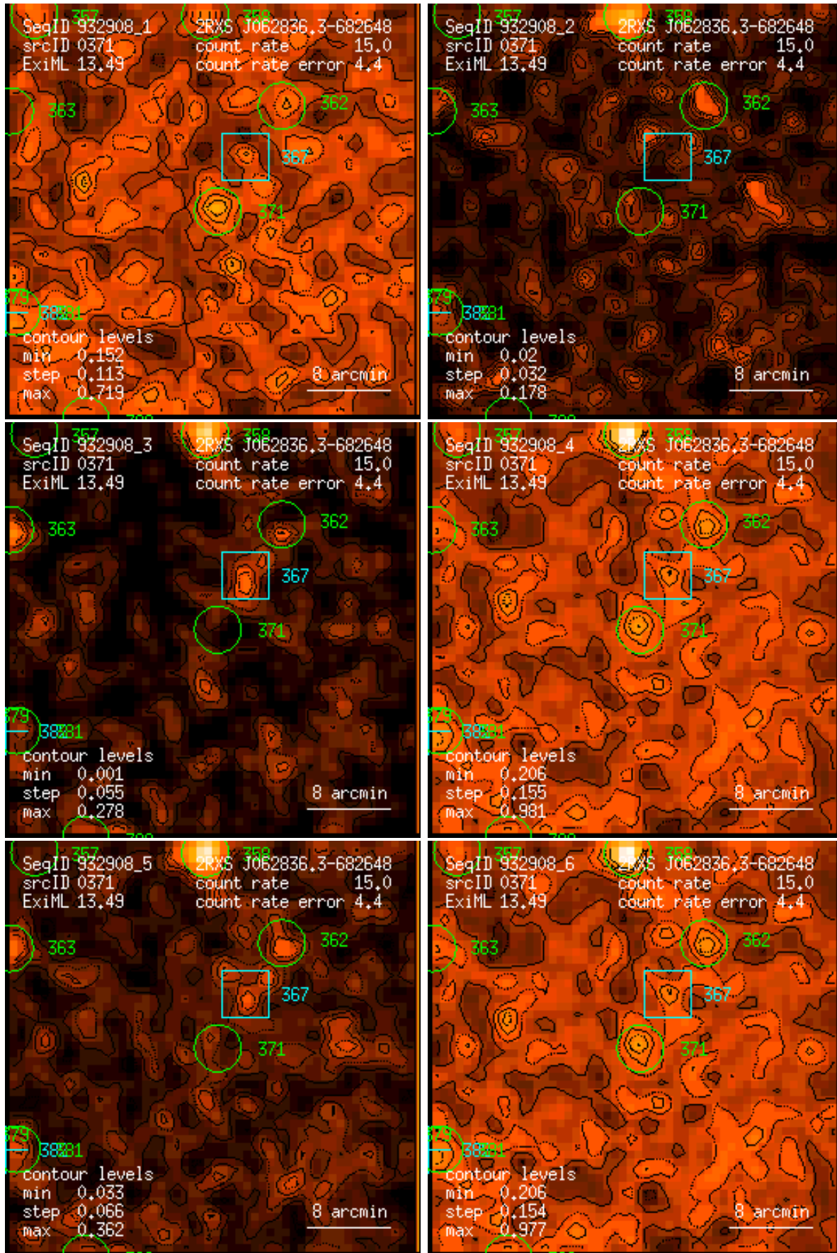
Figure 371: RASS 932908: detection 0371: band rate images, Gaussian filter: (1) PSPPC channels 11 – 41, (2) 52 – 90, (3) 91 – 201, (4) 11 – 235, (5) 52 – 201, (6) 11 – 201. Broad band rates in counts/ks. Band rate contour levels in counts/ks/arcmin 2 .
