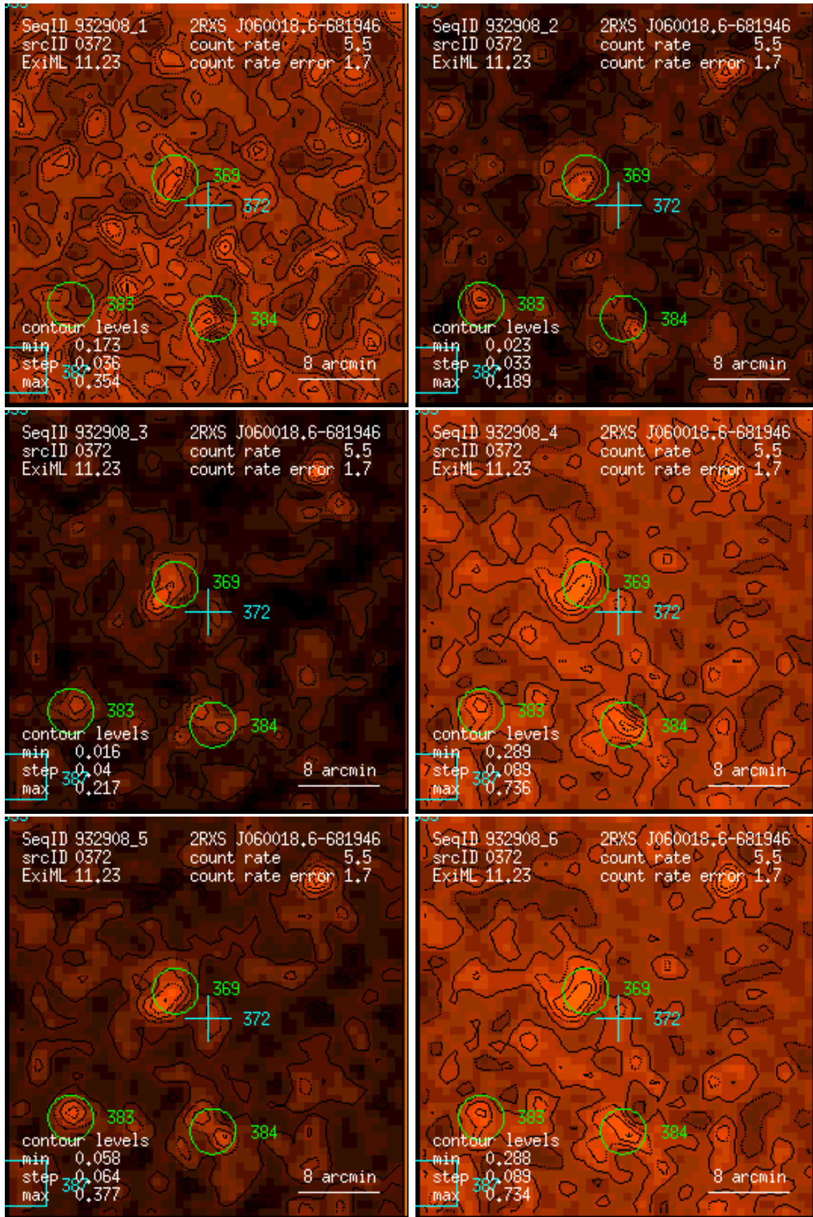
Figure 372: RASS 932908: detection 0372: band rate images, Gaussian filter: (1) PSPC channels 11 – 41, (2) 52 – 90, (3) 91 – 201, (4) 11 – 235, (5) 52 – 201, (6) 11 – 201. Broad band rates in counts/ks. Band rate contour levels in counts/ks/arcmin 2 .
