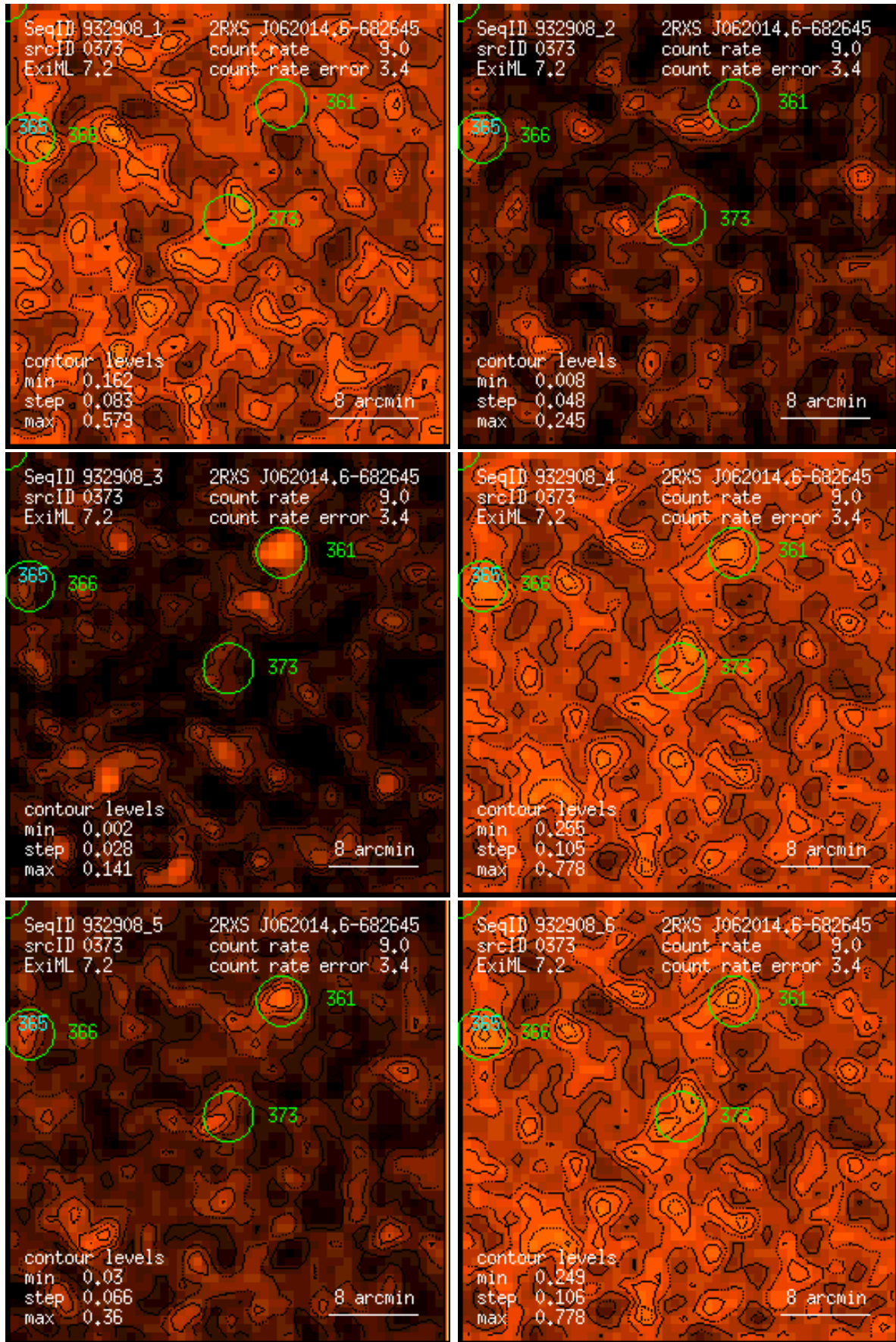
Figure 373: RASS 932908: detection 0373: band rate images, Gaussian filter: (1) PSPC channels 11 – 41, (2) 52 – 90, (3) 91 – 201, (4) 11 – 235, (5) 52 – 201, (6) 11 – 201. Broad band rates in counts/ks. Band rate contour levels in counts/ks/arcmin 2 .
