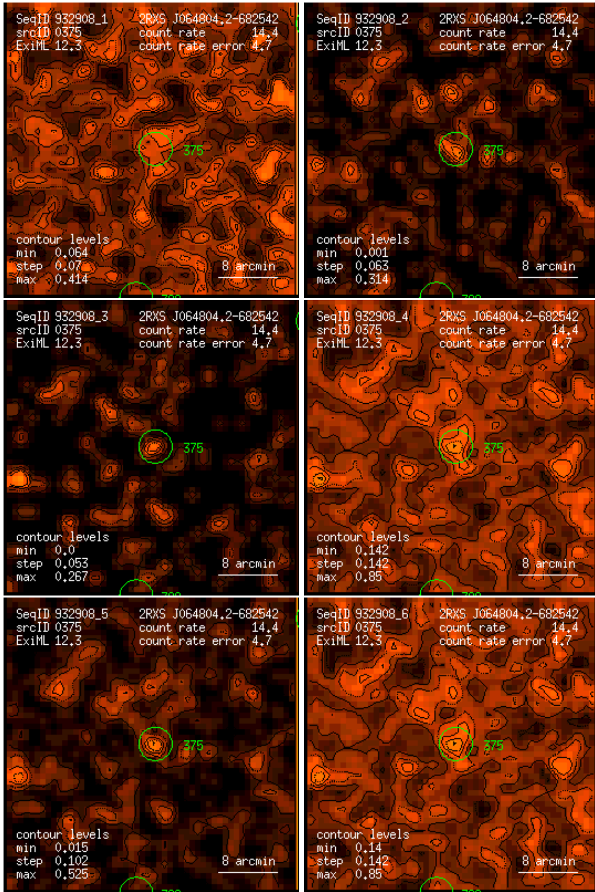
Figure 375: RASS 932908: detection 0375: band rate images, Gaussian filter: (1) PSPC channels 11 – 41, (2) 52 – 90, (3) 91 – 201, (4) 11 – 235, (5) 52 – 201, (6) 11 – 201. Broad band rates in counts/ks. Band rate contour levels in counts/ks/arcmin 2 .
