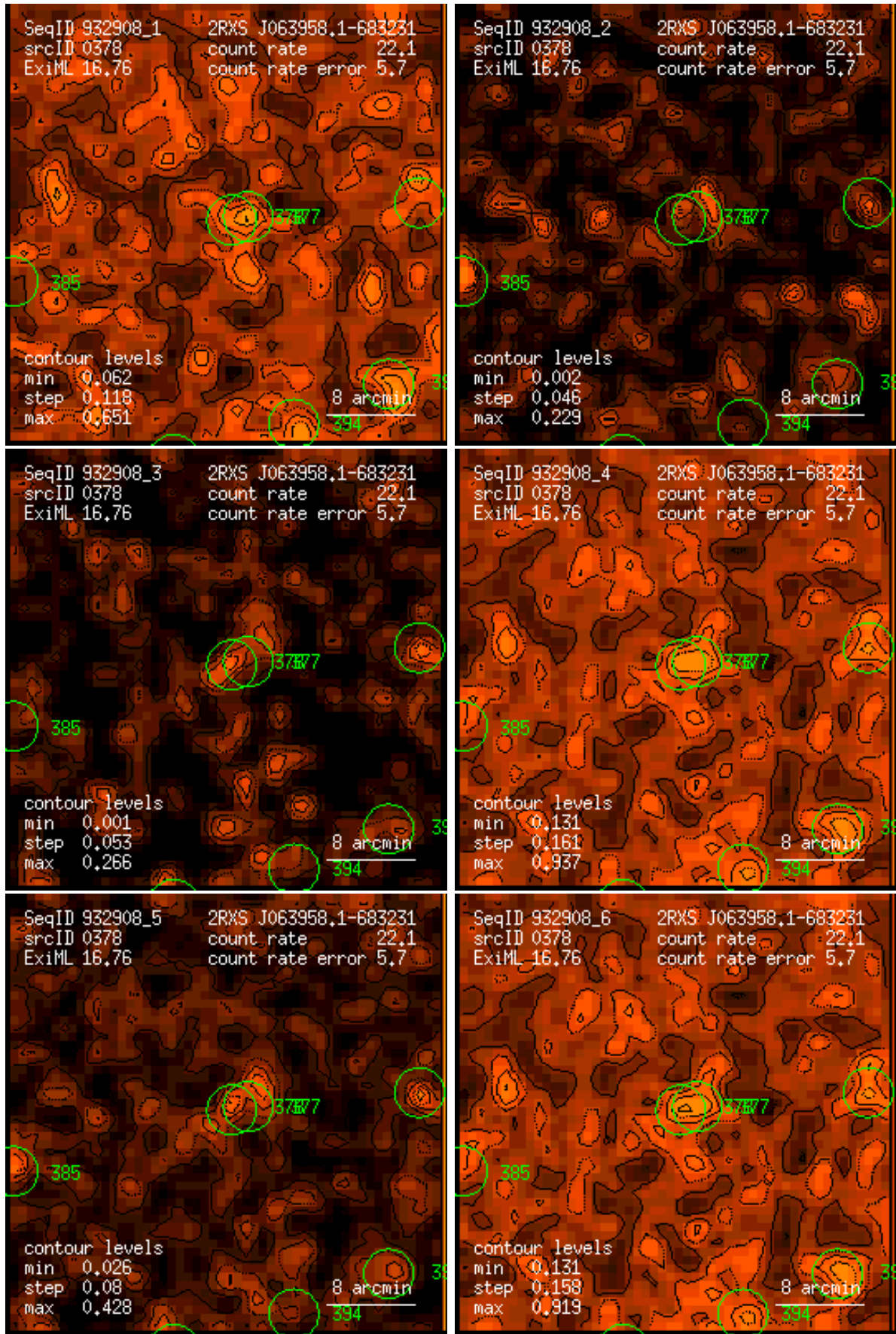
Figure 378: RASS 932908: detection 0378: band rate images, Gaussian filter: (1) PSPC channels 11 – 41, (2) 52 – 90, (3) 91 – 201, (4) 11 – 235, (5) 52 – 201, (6) 11 – 201. Broad band rates in counts/ks. Band rate contour levels in counts/ks/arcmin 2 .
