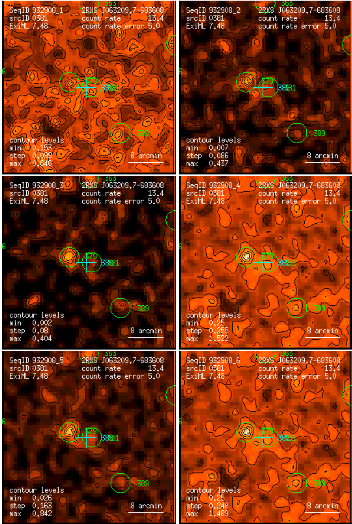
Figure 381: RASS 932908: detection 0381: band rate images, Gaussian filter: (1) PSPC channels 11 – 41, (2) 52 – 90, (3) 91 – 201, (4) 11 – 235, (5) 52 – 201, (6) 11 – 201. Broad band rates in counts/ks. Band rate contour levels in counts/ks/arcmin 2 .
