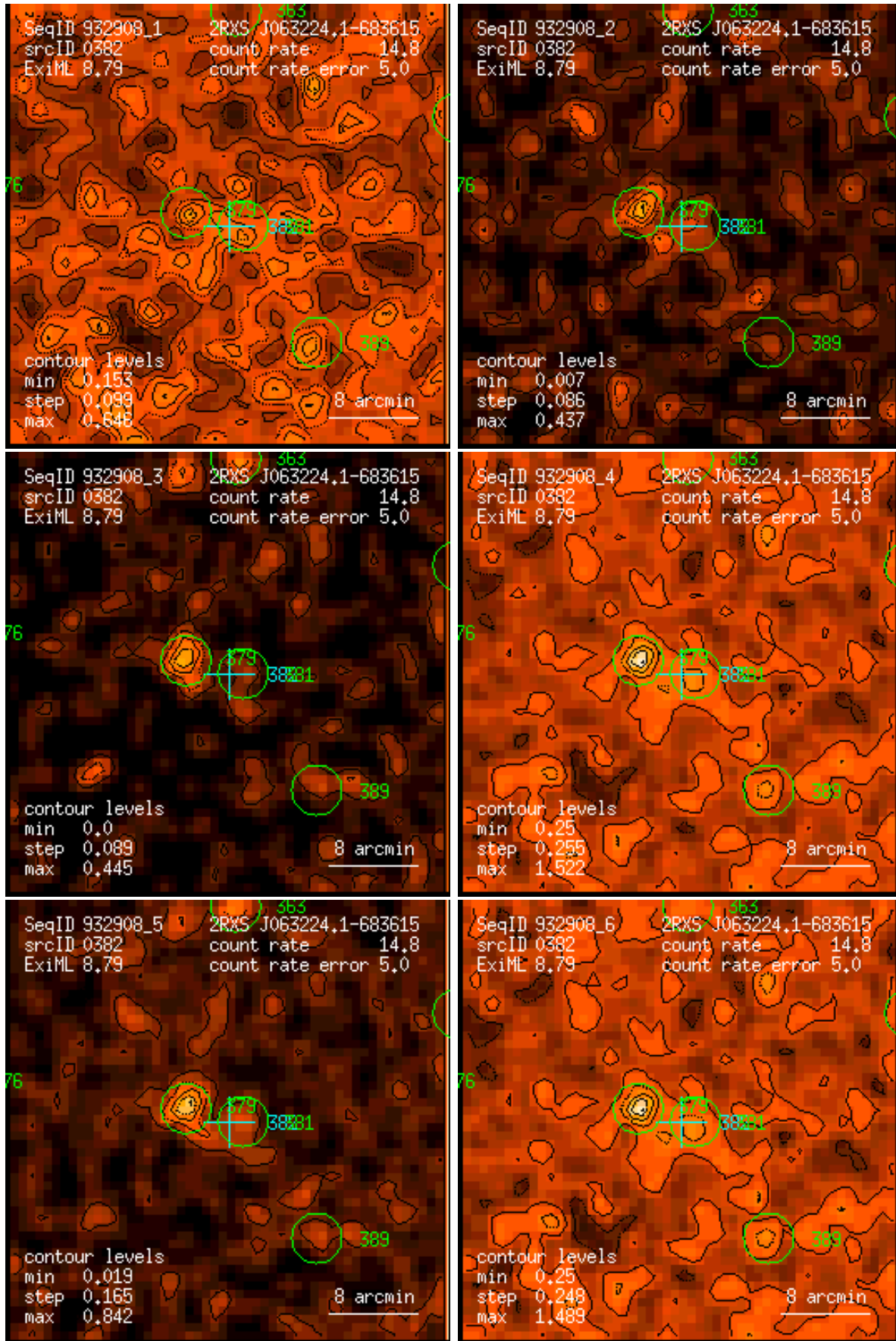
Figure 382: RASS 932908: detection 0382: band rate images, Gaussian filter: (1) PSPC channels 11 – 41, (2) 52 – 90, (3) 91 – 201, (4) 11 – 235, (5) 52 – 201, (6) 11 – 201. Broad band rates in counts/ks. Band rate contour levels in counts/ks/arcmin 2 .
