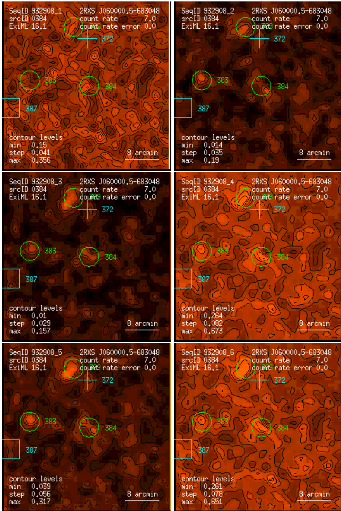
Figure 384: RASS 932908: detection 0384: band rate images, Gaussian filter: (1) PSPC channels 11 – 41, (2) 52 – 90, (3) 91 – 201, (4) 11 – 235, (5) 52 – 201, (6) 11 – 201. Broad band rates in counts/ks. Band rate contour levels in counts/ks/arcmin 2 .
