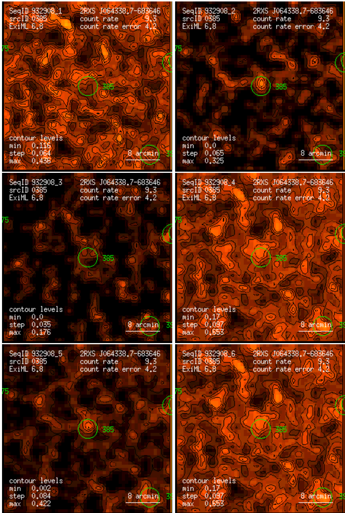
Figure 385: RASS 932908: detection 0385: band rate images, Gaussian filter: (1) PSPC channels 11 – 41, (2) 52 – 90, (3) 91 – 201, (4) 11 – 235, (5) 52 – 201, (6) 11 – 201. Broad band rates in counts/ks. Band rate contour levels in counts/ks/arcmin 2 .
