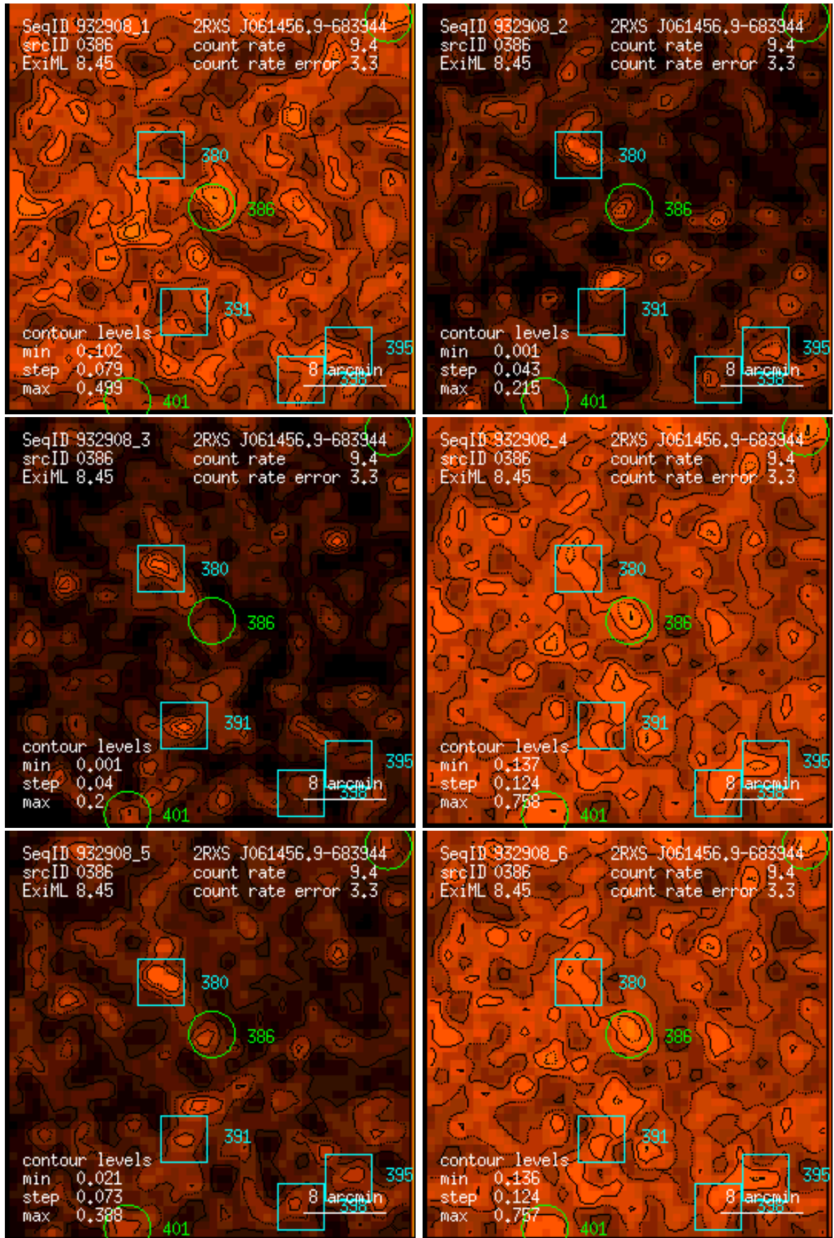
Figure 386: RASS 932908: detection 0386: band rate images, Gaussian filter: (1) PSPC channels 11 – 41, (2) 52 – 90, (3) 91 – 201, (4) 11 – 235, (5) 52 – 201, (6) 11 – 201. Broad band rates in counts/ks. Band rate contour levels in counts/ks/arcmin 2 .
