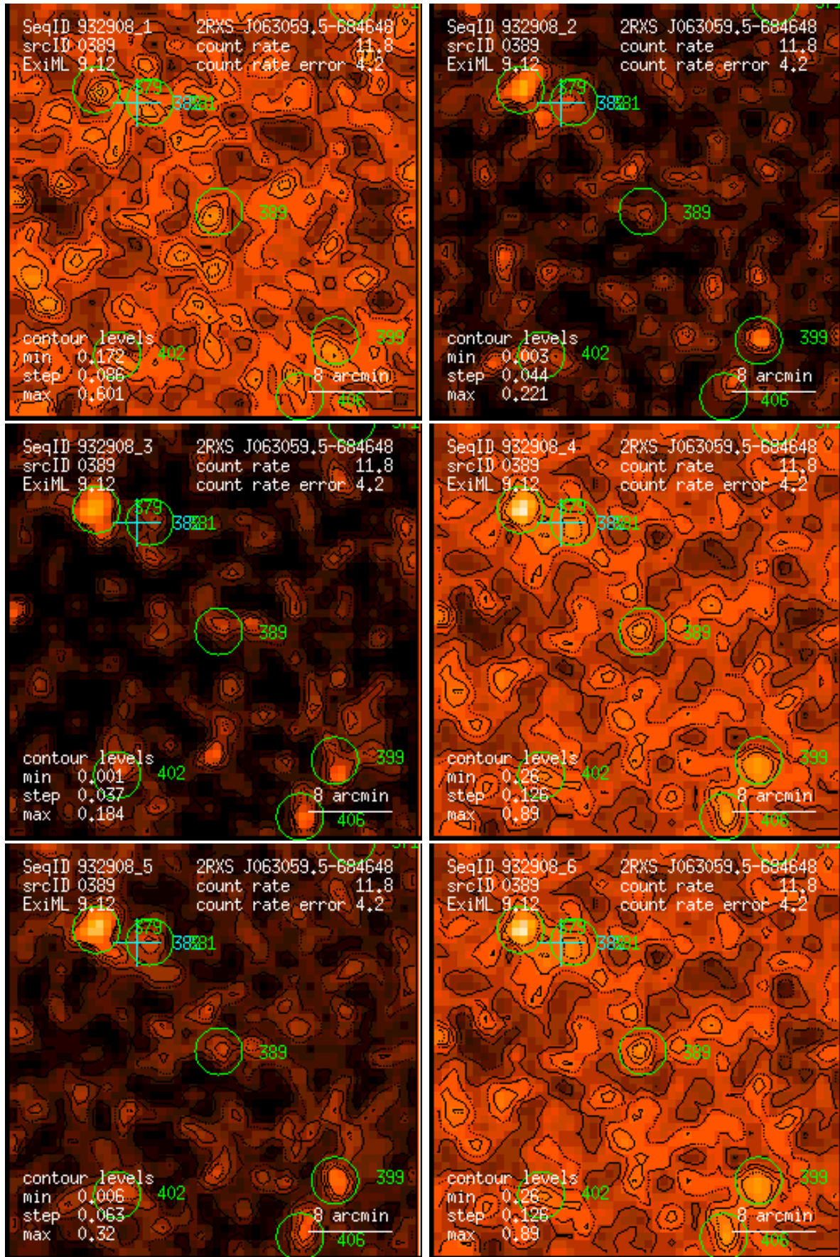
Figure 389: RASS 932908: detection 0389: band rate images, Gaussian filter: (1) PSPC channels 11 – 41, (2) 52 – 90, (3) 91 – 201, (4) 11 – 235, (5) 52 – 201, (6) 11 – 201. Broad band rates in counts/ks. Band rate contour levels in counts/ks/arcmin 2 .
