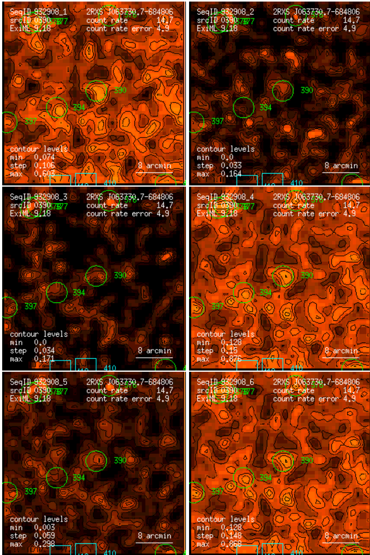
Figure 390: RASS 932908: detection 0390: band rate images, Gaussian filter: (1) PSPC channels 11 – 41, (2) 52 – 90, (3) 91 – 201, (4) 11 – 235, (5) 52 – 201, (6) 11 – 201. Broad band rates in counts/ks. Band rate contour levels in counts/ks/arcmin 2 .
