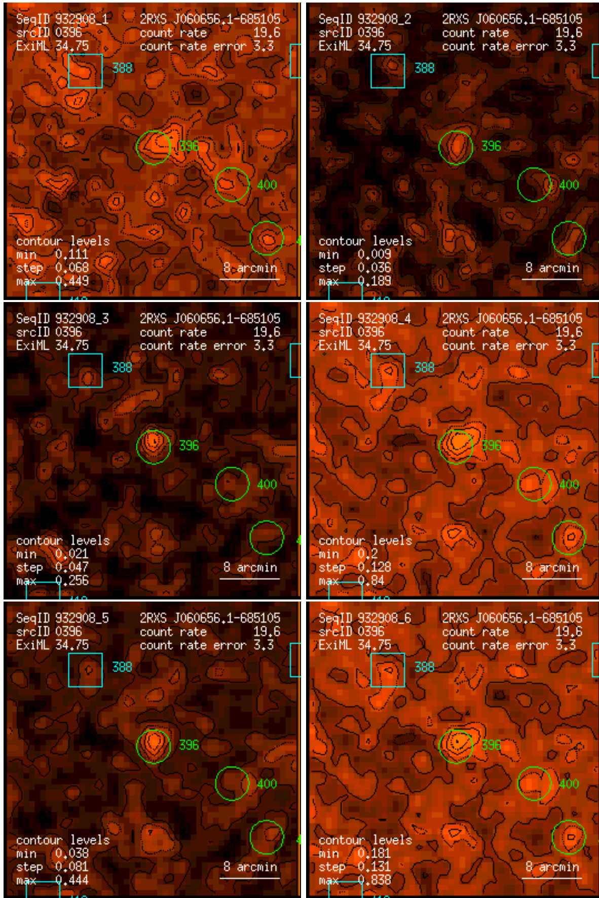
Figure 396: RASS 932908: detection 0396: band rate images, Gaussian filter: (1) PSPC channels 11 – 41, (2) 52 – 90, (3) 91 – 201, (4) 11 – 235, (5) 52 – 201, (6) 11 – 201. Broad band rates in counts/ks. Band rate contour levels in counts/ks/arcmin 2 .
