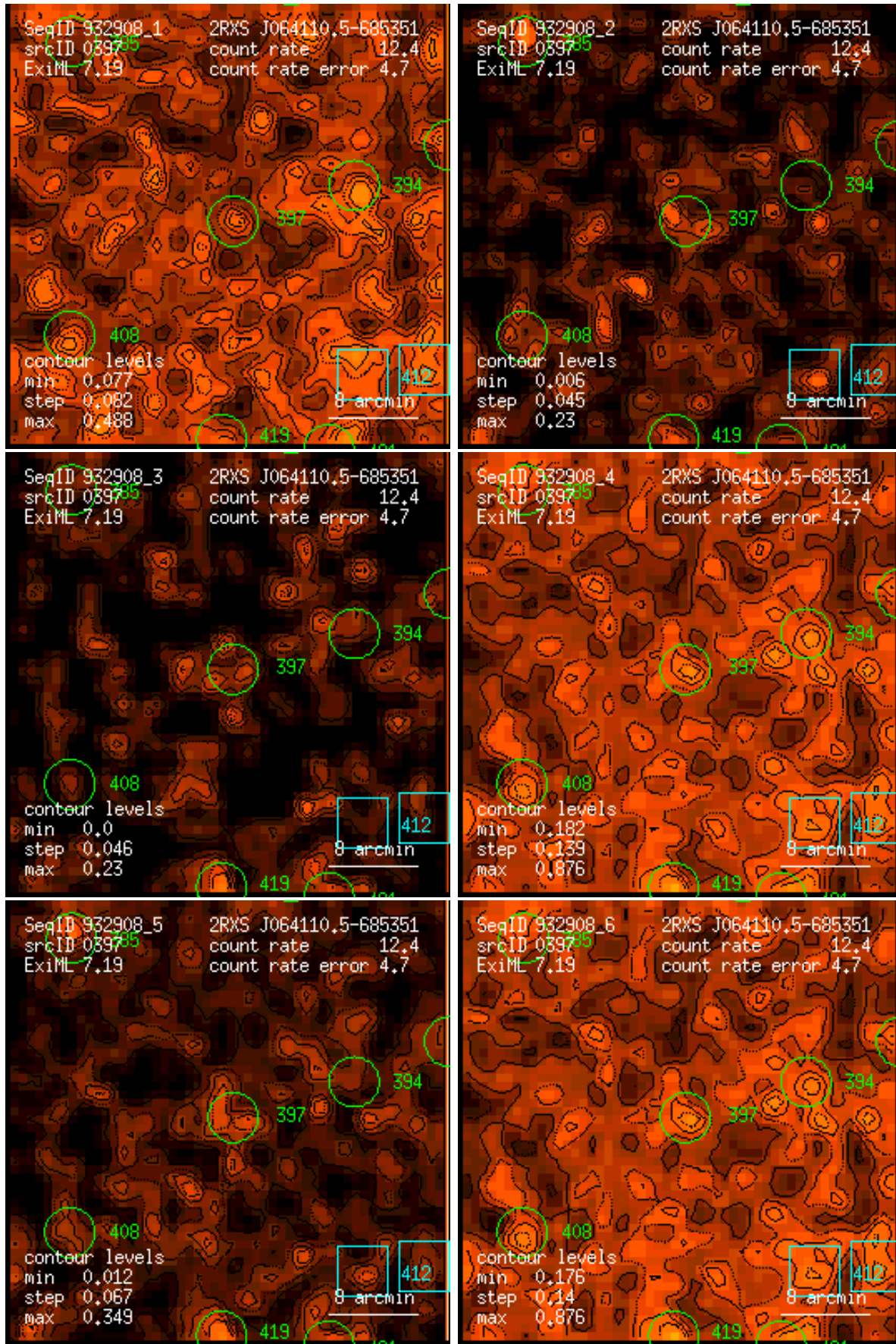
Figure 397: RASS 932908: detection 0397: band rate images, Gaussian filter: (1) PSPC channels 11 – 41, (2) 52 – 90, (3) 91 – 201, (4) 11 – 235, (5) 52 – 201, (6) 11 – 201. Broad band rates in counts/ks. Band rate contour levels in counts/ks/arcmin 2 .
