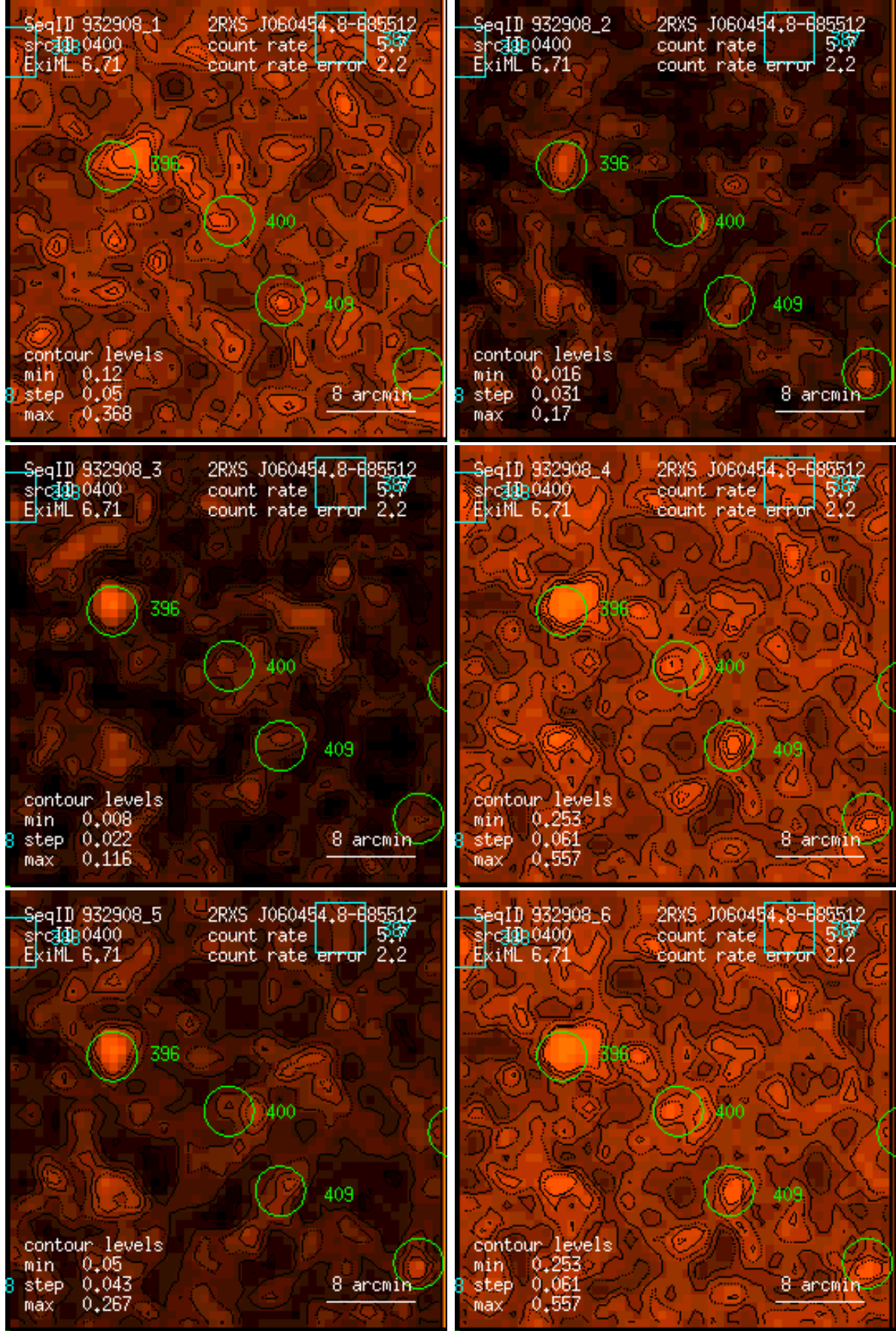
Figure 400: RASS 932908: detection 0400: band rate images, Gaussian filter: (1) PSPC channels 11 – 41, (2) 52 – 90, (3) 91 – 201, (4) 11 – 235, (5) 52 – 201, (6) 11 – 201. Broad band rates in counts/ks. Band rate contour levels in counts/ks/arcmin 2 .
