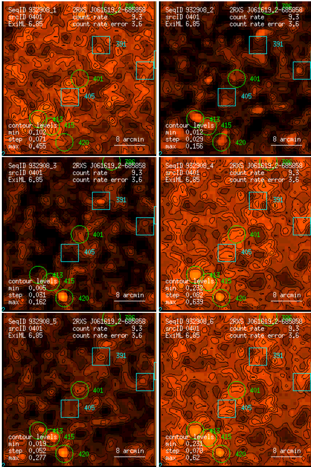
Figure 401: RASS 932908: detection 0401: band rate images, Gaussian filter: (1) PSPC channels 11 – 41, (2) 52 – 90, (3) 91 – 201, (4) 11 – 235, (5) 52 – 201, (6) 11 – 201. Broad band rates in counts/ks. Band rate contour levels in counts/ks/arcmin 2 .
