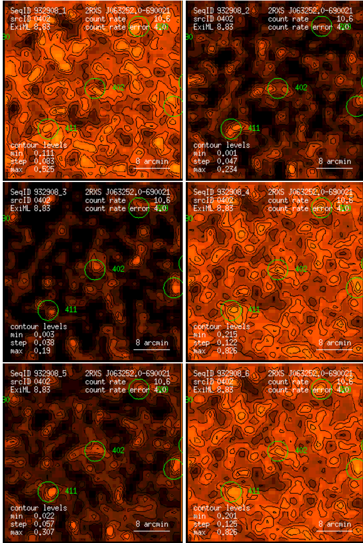
Figure 402: RASS 932908: detection 0402: band rate images, Gaussian filter: (1) PSPC channels 11 – 41, (2) 52 – 90, (3) 91 – 201, (4) 11 – 235, (5) 52 – 201, (6) 11 – 201. Broad band rates in counts/ks. Band rate contour levels in counts/ks/arcmin 2 .
