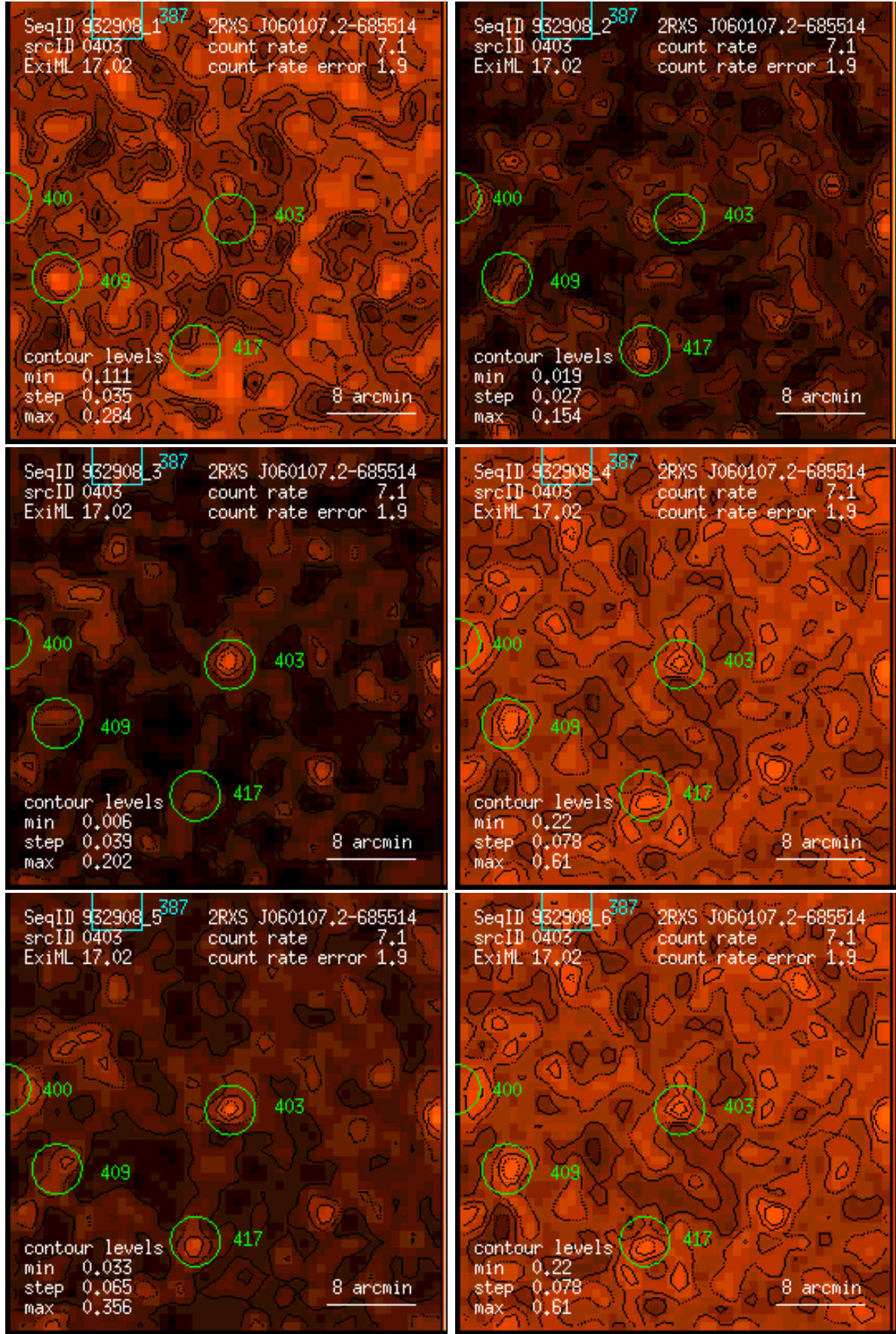
Figure 403: RASS 932908: detection 0403: band rate images, Gaussian filter: (1) PSPC channels 11 – 41, (2) 52 – 90, (3) 91 – 201, (4) 11 – 235, (5) 52 – 201, (6) 11 – 201. Broad band rates in counts/ks. Band rate contour levels in counts/ks/arcmin 2 .
