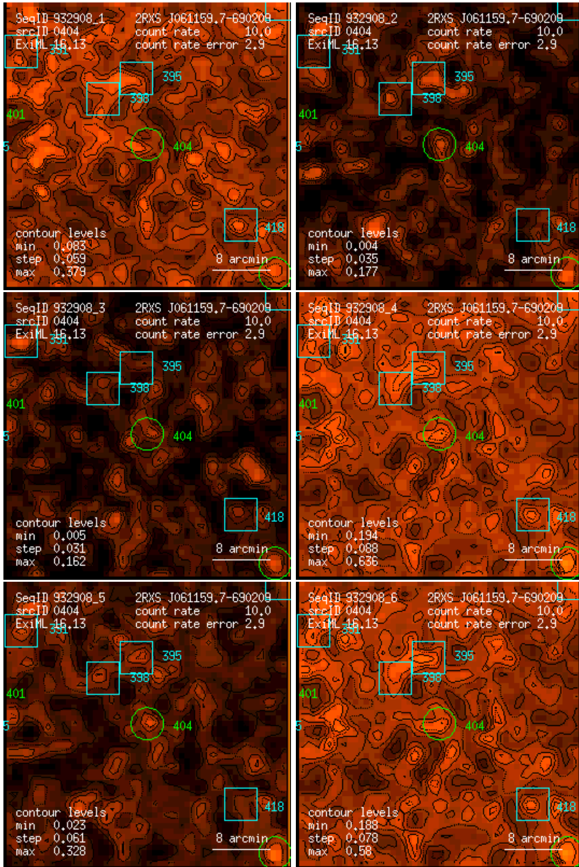
Figure 404: RASS 932908: detection 0404: band rate images, Gaussian filter: (1) PSPC channels 11 – 41, (2) 52 – 90, (3) 91 – 201, (4) 11 – 235, (5) 52 – 201, (6) 11 – 201. Broad band rates in counts/ks. Band rate contour levels in counts/ks/arcmin 2 .
