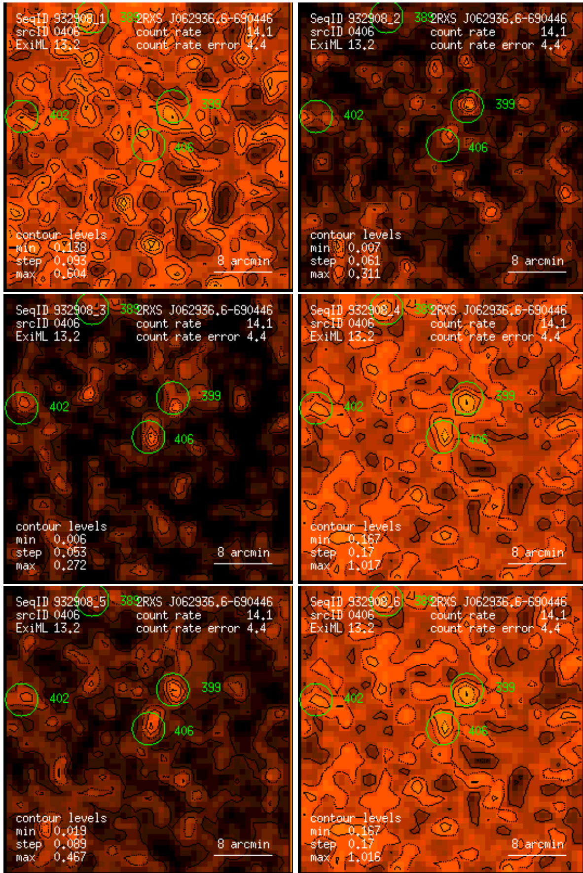
Figure 406: RASS 932908: detection 0406: band rate images, Gaussian filter: (1) PSPC channels 11 – 41, (2) 52 – 90, (3) 91 – 201, (4) 11 – 235, (5) 52 – 201, (6) 11 – 201. Broad band rates in counts/ks. Band rate contour levels in counts/ks/arcmin 2 .
