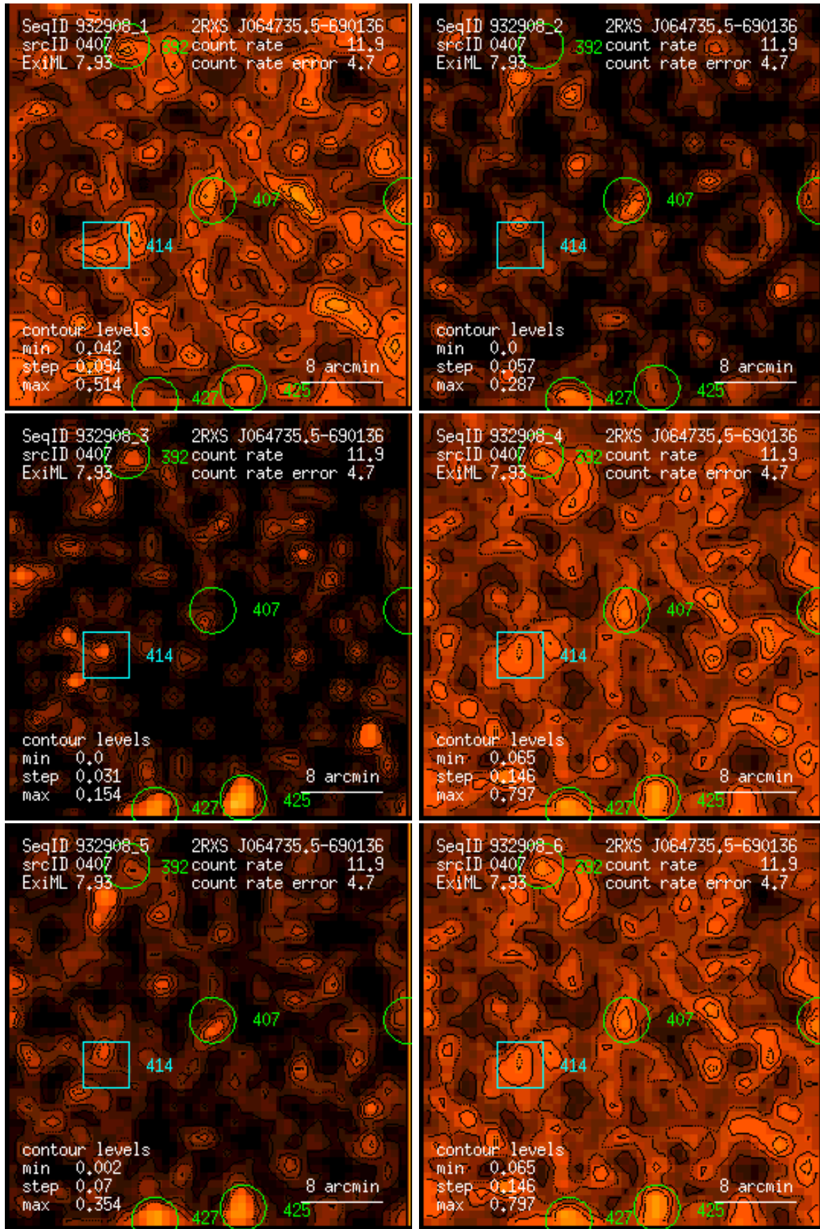
Figure 407: RASS 932908: detection 0407: band rate images, Gaussian filter: (1) PSPC channels 11 – 41, (2) 52 – 90, (3) 91 – 201, (4) 11 – 235, (5) 52 – 201, (6) 11 – 201. Broad band rates in counts/ks. Band rate contour levels in counts/ks/arcmin 2 .
