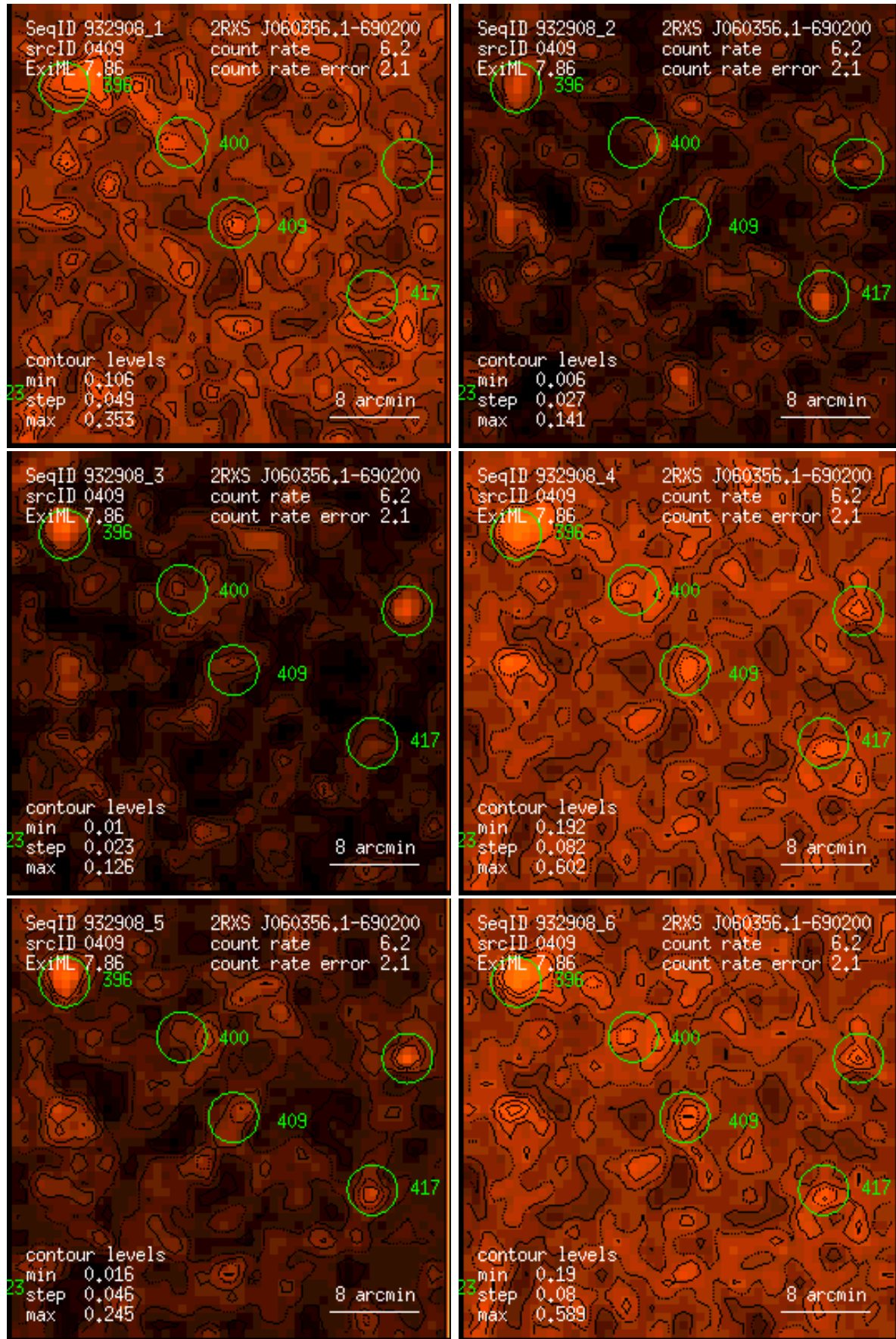
Figure 409: RASS 932908: detection 0409: band rate images, Gaussian filter: (1) PSPC channels 11 – 41, (2) 52 – 90, (3) 91 – 201, (4) 11 – 235, (5) 52 – 201, (6) 11 – 201. Broad band rates in counts/ks. Band rate contour levels in counts/ks/arcmin 2 .
