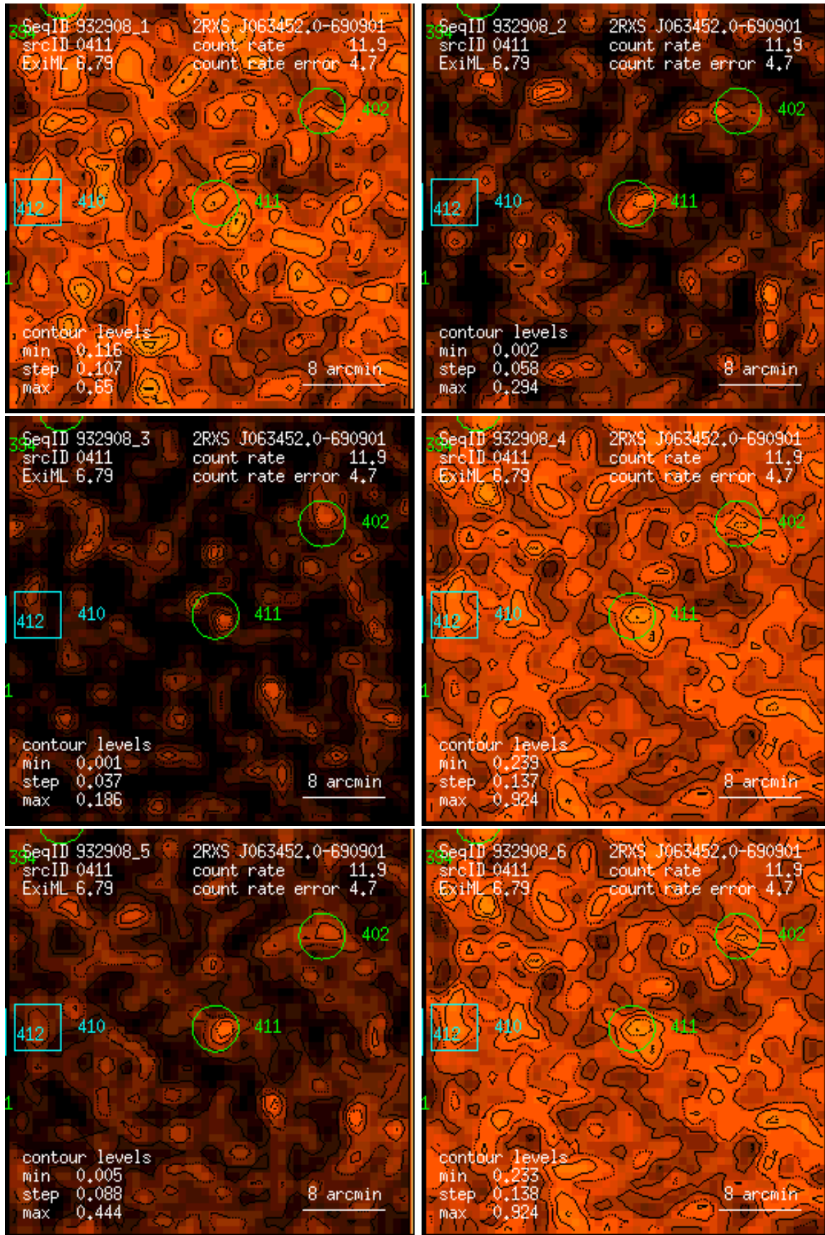
Figure 411: RASS 932908: detection 0411: band rate images, Gaussian filter: (1) PSPC channels 11 – 41, (2) 52 – 90, (3) 91 – 201, (4) 11 – 235, (5) 52 – 201, (6) 11 – 201. Broad band rates in counts/ks. Band rate contour levels in counts/ks/arcmin 2 .
