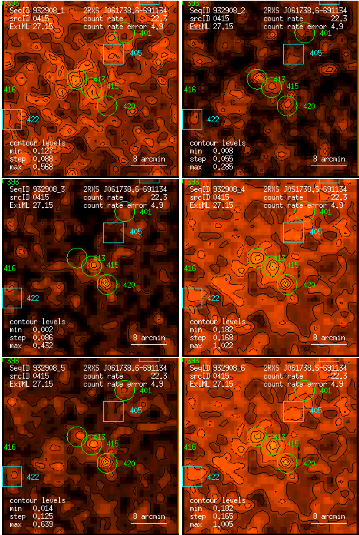
Figure 415: RASS 932908: detection 0415: band rate images, Gaussian filter: (1) PSPC channels 11 – 41, (2) 52 – 90, (3) 91 – 201, (4) 11 – 235, (5) 52 – 201, (6) 11 – 201. Broad band rates in counts/ks. Band rate contour levels in counts/ks/arcmin 2 .
