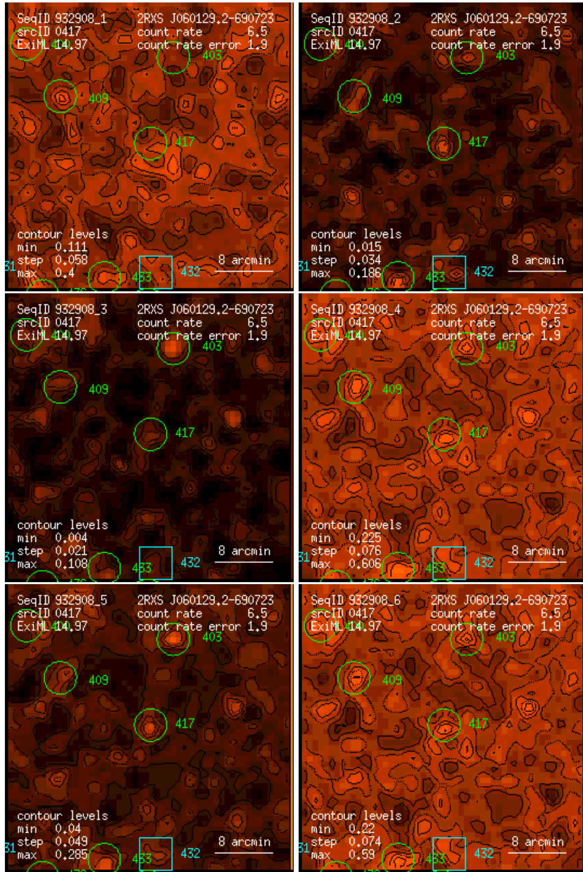
Figure 417: RASS 932908: detection 0417: band rate images, Gaussian filter: (1) PSPC channels 11 – 41, (2) 52 – 90, (3) 91 – 201, (4) 11 – 235, (5) 52 – 201, (6) 11 – 201. Broad band rates in counts/ks. Band rate contour levels in counts/ks/arcmin 2 .
