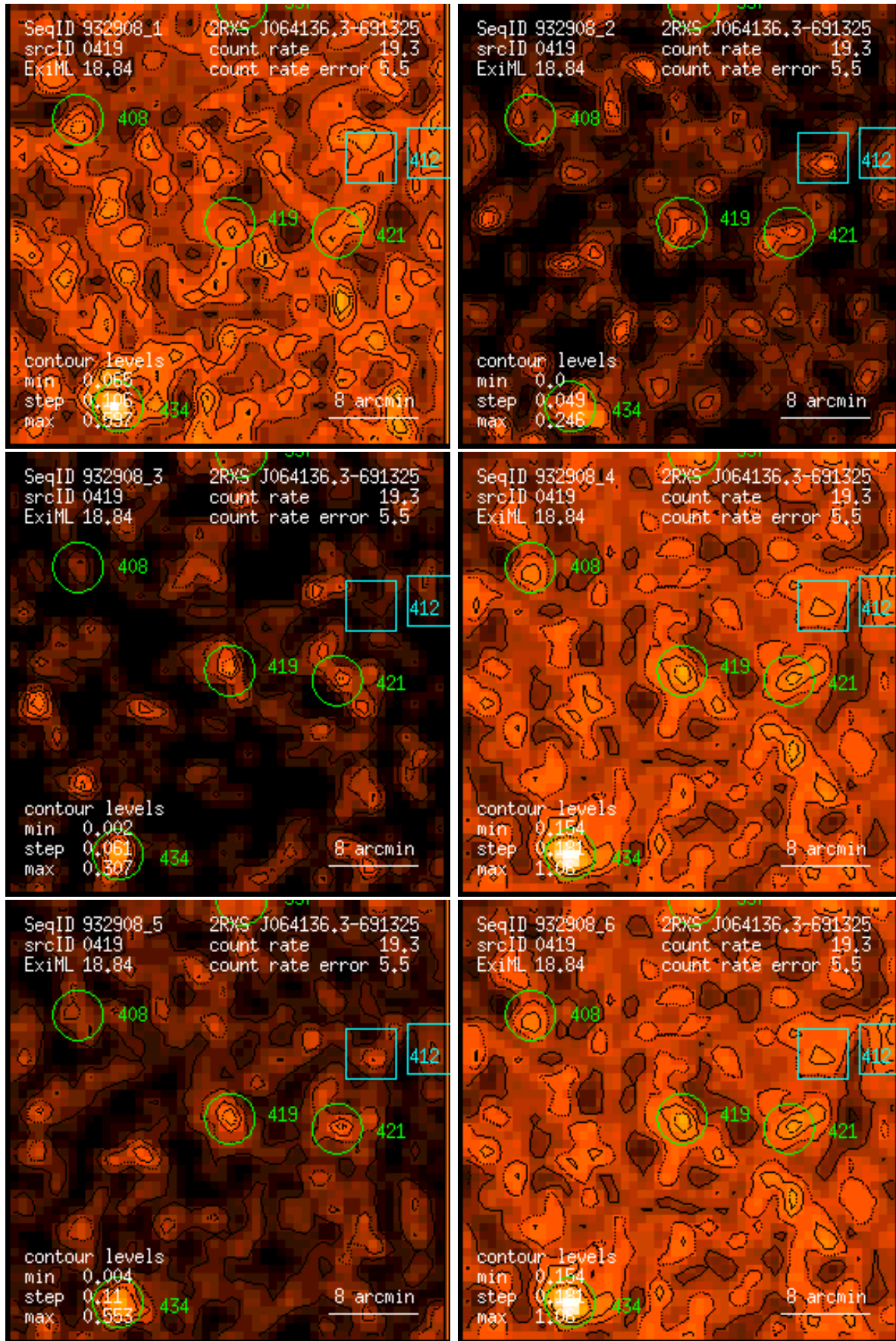
Figure 419: RASS 932908: detection 0419: band rate images, Gaussian filter: (1) PSPC channels 11 – 41, (2) 52 – 90, (3) 91 – 201, (4) 11 – 235, (5) 52 – 201, (6) 11 – 201. Broad band rates in counts/ks. Band rate contour levels in counts/ks/arcmin 2 .
