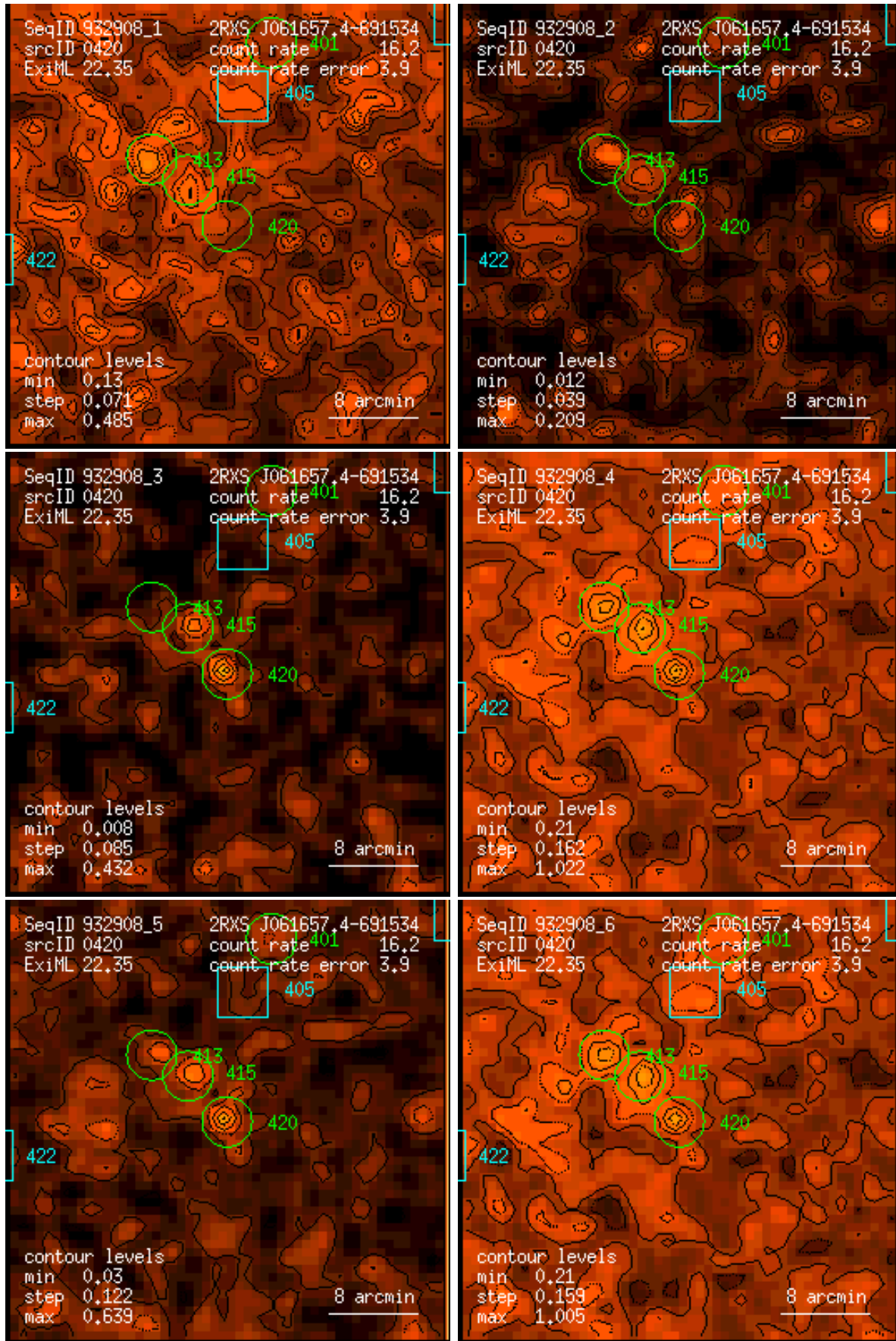
Figure 420: RASS 932908: detection 0420: band rate images, Gaussian filter: (1) PSPC channels 11 – 41, (2) 52 – 90, (3) 91 – 201, (4) 11 – 235, (5) 52 – 201, (6) 11 – 201. Broad band rates in counts/ks. Band rate contour levels in counts/ks/arcmin 2 .
