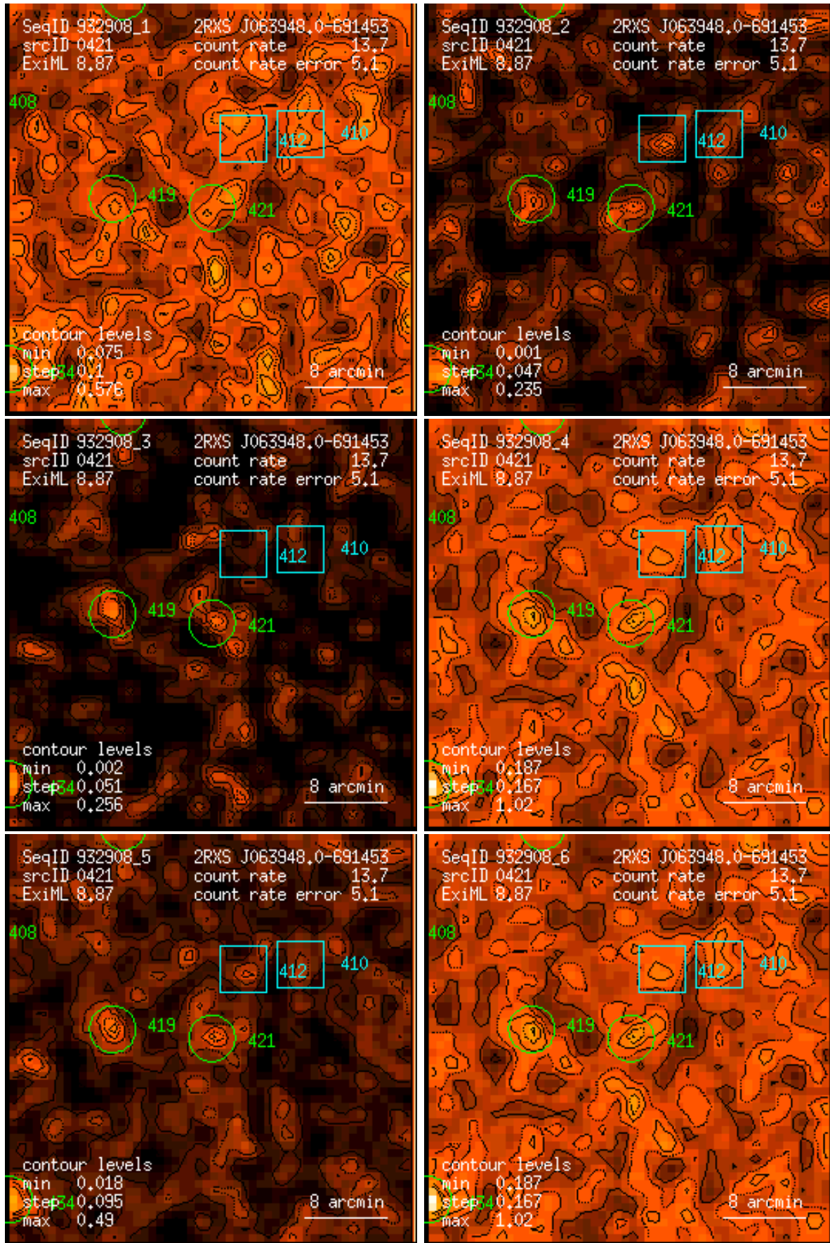
Figure 421: RASS 932908: detection 0421: band rate images, Gaussian filter: (1) PSPC channels 11 – 41, (2) 52 – 90, (3) 91 – 201, (4) 11 – 235, (5) 52 – 201, (6) 11 – 201. Broad band rates in counts/ks. Band rate contour levels in counts/ks/arcmin 2 .
