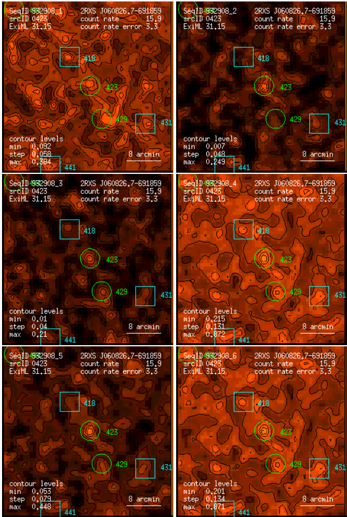
Figure 423: RASS 932908: detection 0423: band rate images, Gaussian filter: (1) PSPC channels 11 – 41, (2) 52 – 90, (3) 91 – 201, (4) 11 – 235, (5) 52 – 201, (6) 11 – 201. Broad band rates in counts/ks. Band rate contour levels in counts/ks/arcmin 2 .
