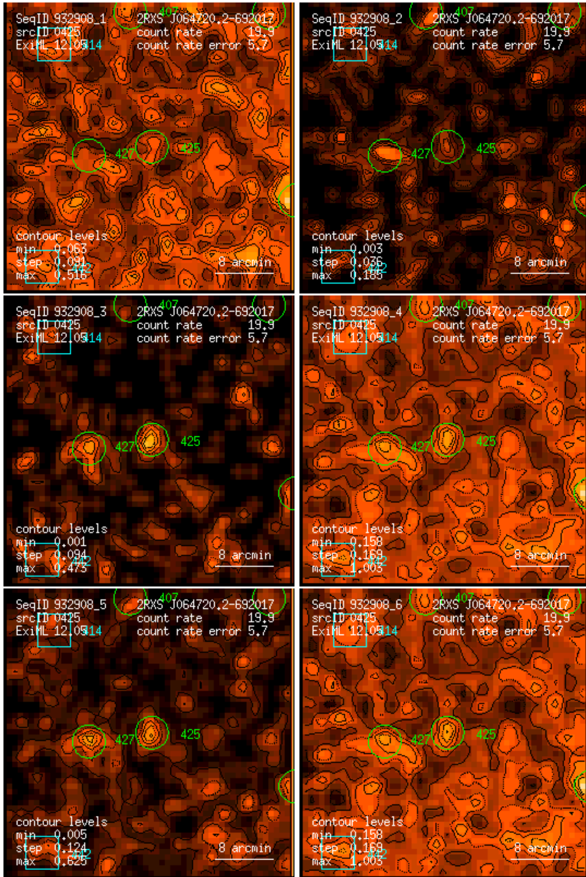
Figure 425: RASS 932908: detection 0425: band rate images, Gaussian filter: (1) PSPC channels 11 – 41, (2) 52 – 90, (3) 91 – 201, (4) 11 – 235, (5) 52 – 201, (6) 11 – 201. Broad band rates in counts/ks. Band rate contour levels in counts/ks/arcmin 2 .
