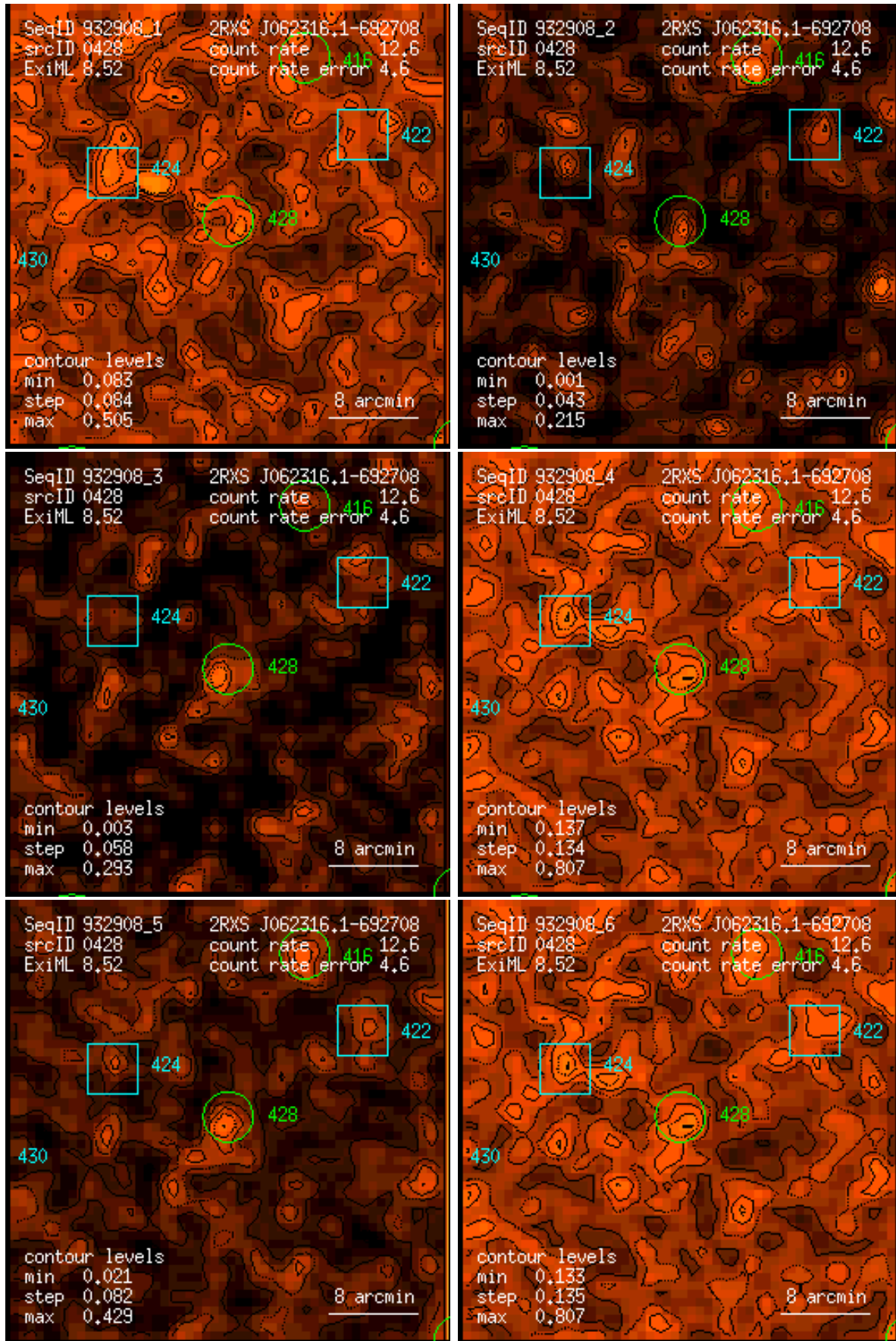
Figure 428: RASS 932908: detection 0428: band rate images, Gaussian filter: (1) PSPC channels 11 – 41, (2) 52 – 90, (3) 91 – 201, (4) 11 – 235, (5) 52 – 201, (6) 11 – 201. Broad band rates in counts/ks. Band rate contour levels in counts/ks/arcmin 2 .
