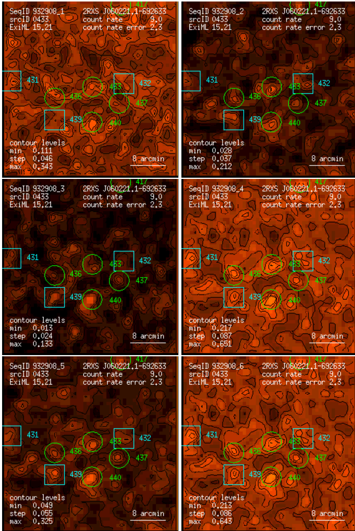
Figure 433: RASS 932908: detection 0433: band rate images, Gaussian filter: (1) PSPC channels 11 – 41, (2) 52 – 90, (3) 91 – 201, (4) 11 – 235, (5) 52 – 201, (6) 11 – 201. Broad band rates in counts/ks. Band rate contour levels in counts/ks/arcmin 2 .
