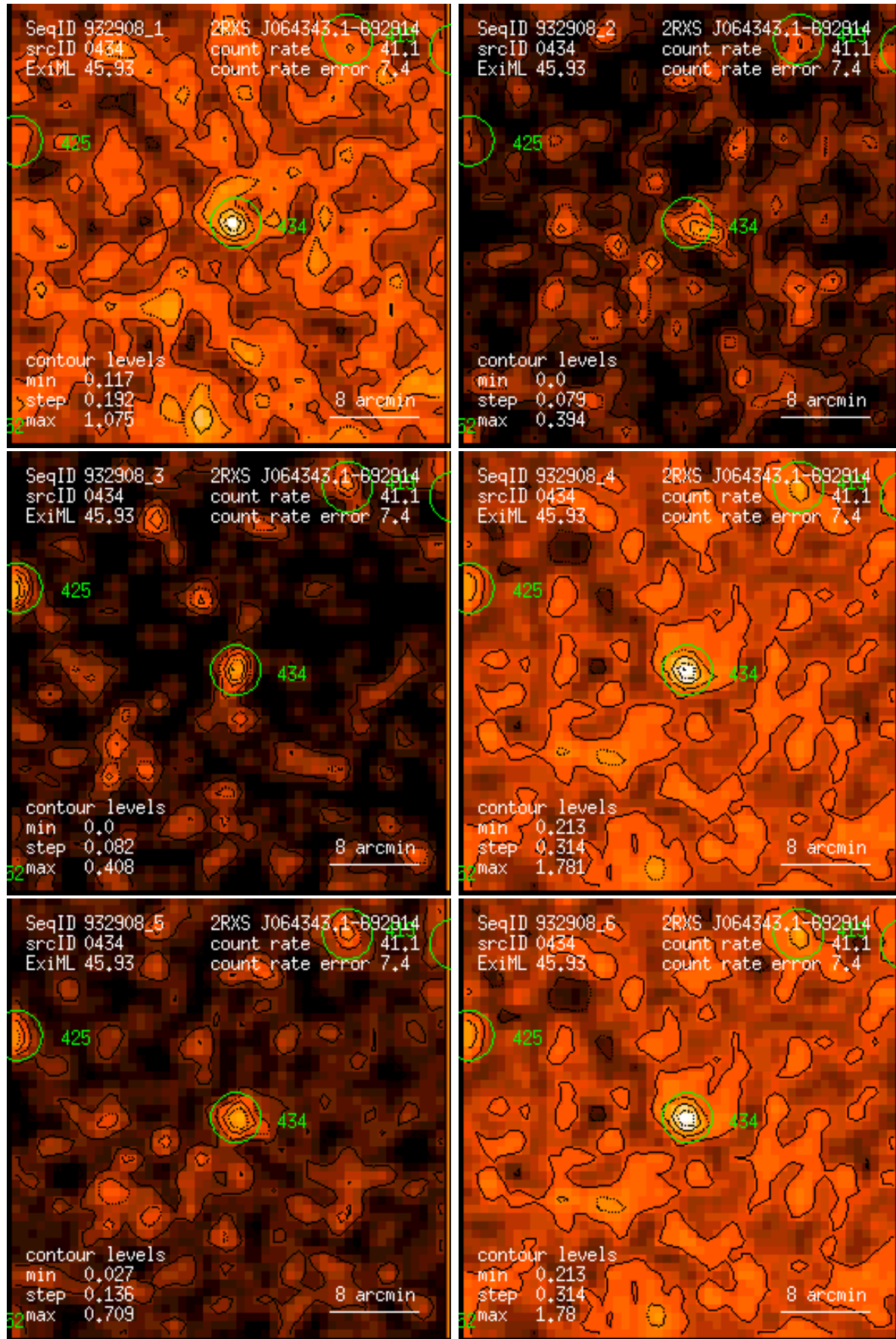
Figure 434: RASS 932908: detection 0434: band rate images, Gaussian filter: (1) PSPC channels 11 – 41, (2) 52 – 90, (3) 91 – 201, (4) 11 – 235, (5) 52 – 201, (6) 11 – 201. Broad band rates in counts/ks. Band rate contour levels in counts/ks/arcmin 2 .
