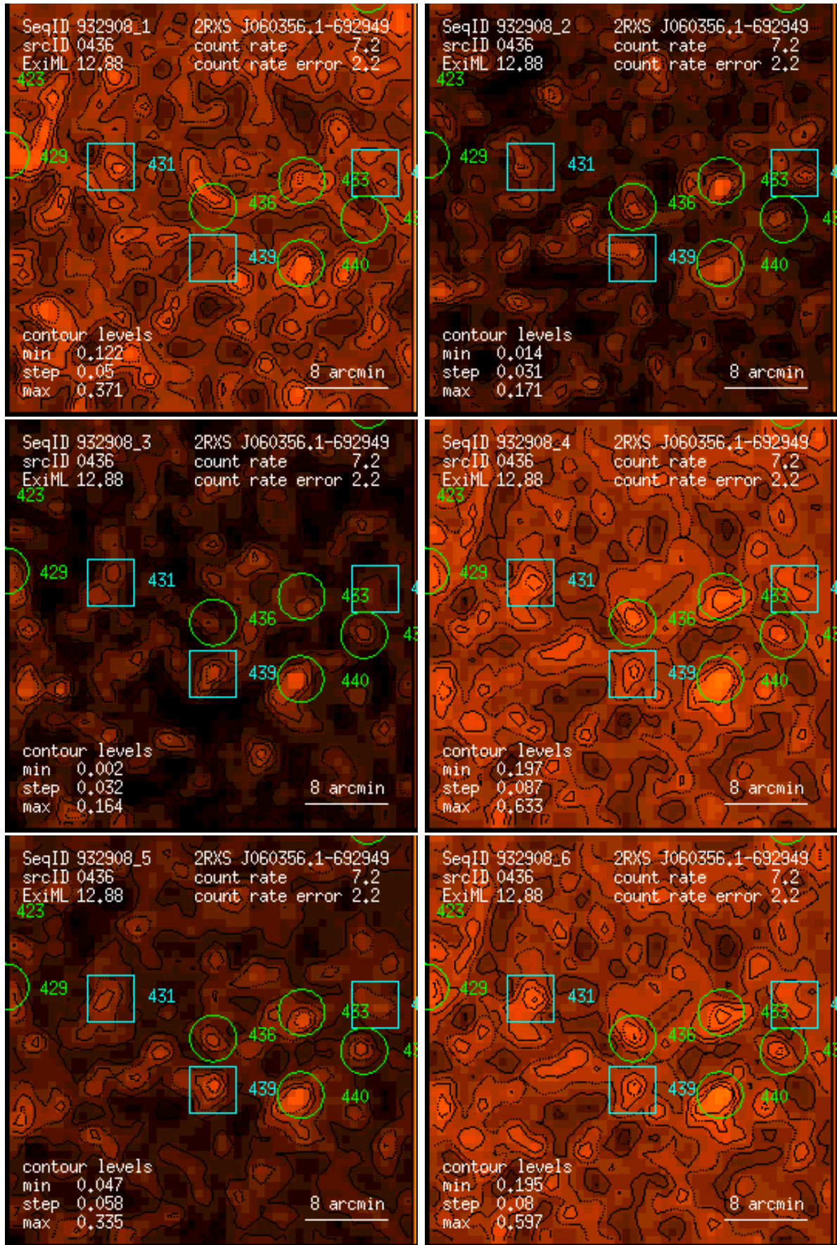
Figure 436: RASS 932908: detection 0436: band rate images, Gaussian filter: (1) PSPC channels 11 – 41, (2) 52 – 90, (3) 91 – 201, (4) 11 – 235, (5) 52 – 201, (6) 11 – 201. Broad band rates in counts/ks. Band rate contour levels in counts/ks/arcmin 2 .
