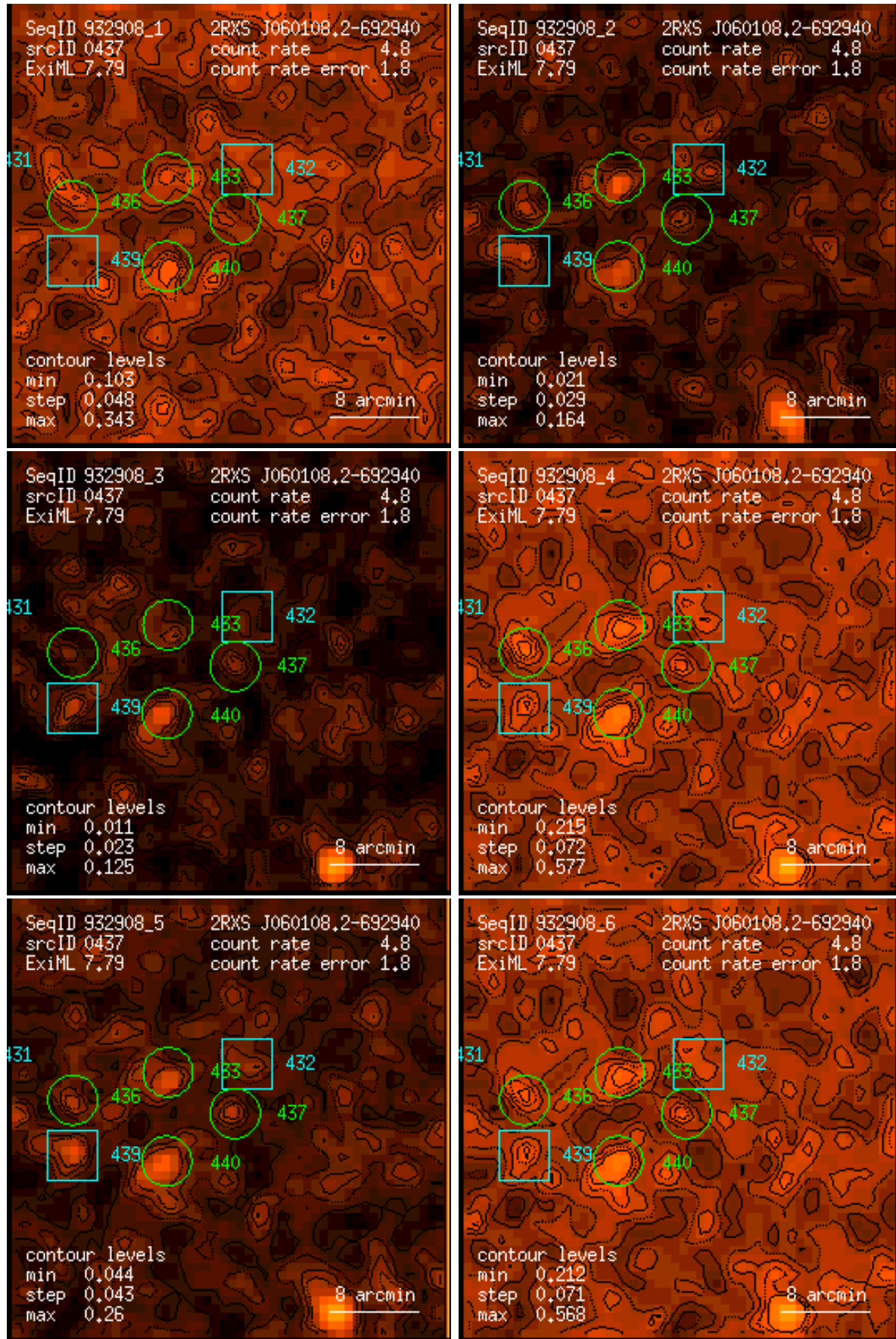
Figure 437: RASS 932908: detection 0437: band rate images, Gaussian filter: (1) PSPC channels 11 – 41, (2) 52 – 90, (3) 91 – 201, (4) 11 – 235, (5) 52 – 201, (6) 11 – 201. Broad band rates in counts/ks. Band rate contour levels in counts/ks/arcmin 2 .
