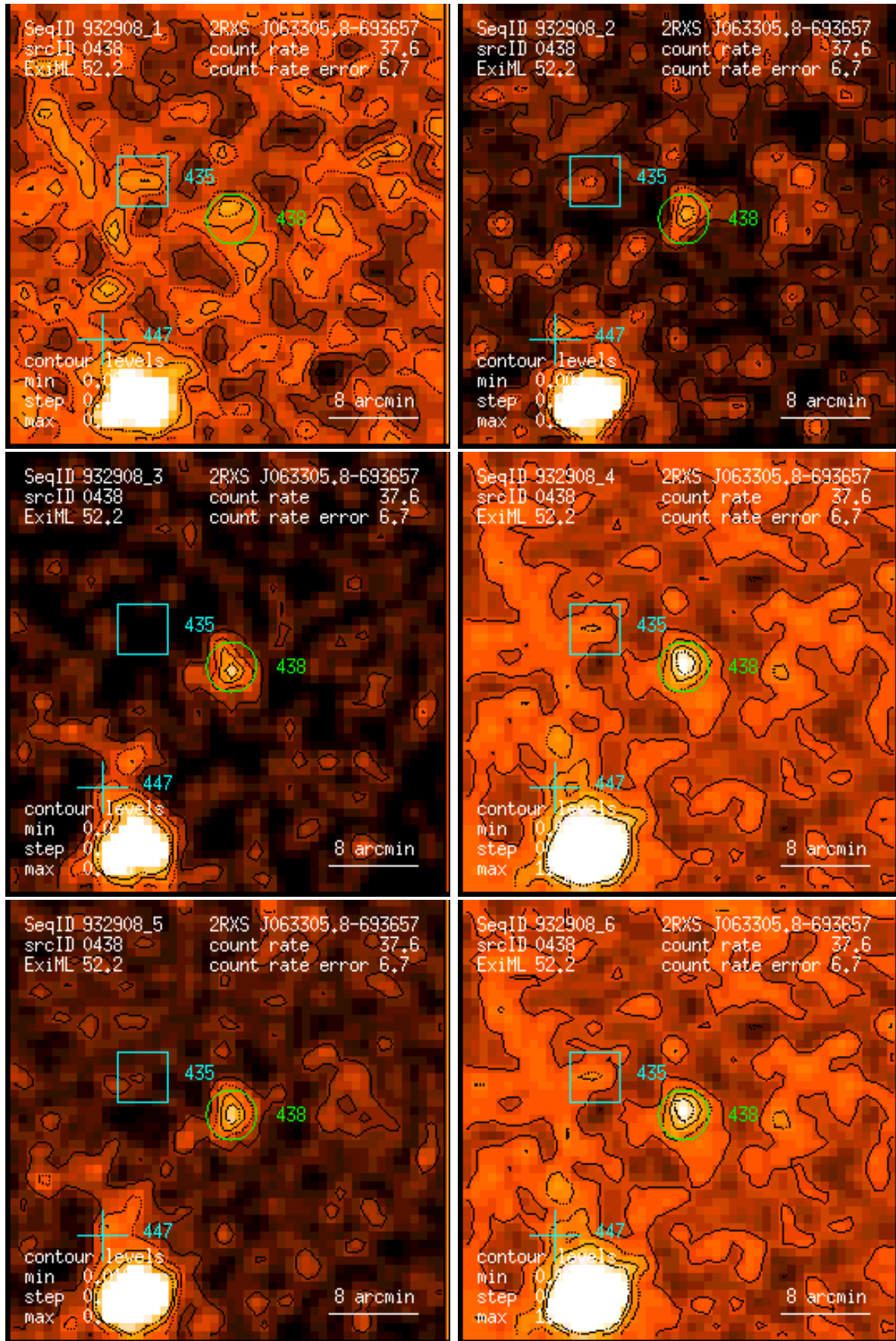
Figure 438: RASS 932908: detection 0438: band rate images, Gaussian filter: (1) PSPC channels 11 – 41, (2) 52 – 90, (3) 91 – 201, (4) 11 – 235, (5) 52 – 201, (6) 11 – 201. Broad band rates in counts/ks. Band rate contour levels in counts/ks/arcmin 2 .
