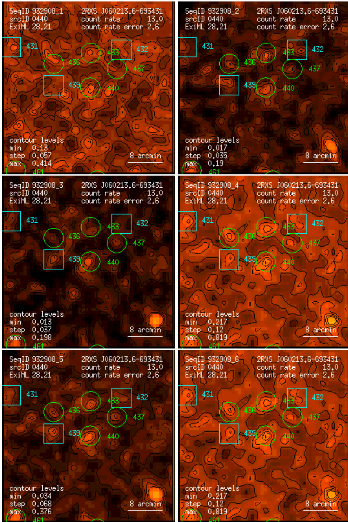
Figure 440: RASS 932908: detection 0440: band rate images, Gaussian filter: (1) PSPC channels 11 – 41, (2) 52 – 90, (3) 91 – 201, (4) 11 – 235, (5) 52 – 201, (6) 11 – 201. Broad band rates in counts/ks. Band rate contour levels in counts/ks/arcmin 2 .
