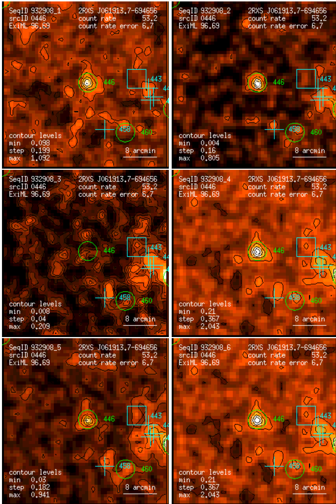
Figure 446: RASS 932908: detection 0446: band rate images, Gaussian filter: (1) PSPC channels 11 – 41, (2) 52 – 90, (3) 91 – 201, (4) 11 – 235, (5) 52 – 201, (6) 11 – 201. Broad band rates in counts/ks. Band rate contour levels in counts/ks/arcmin 2 .
