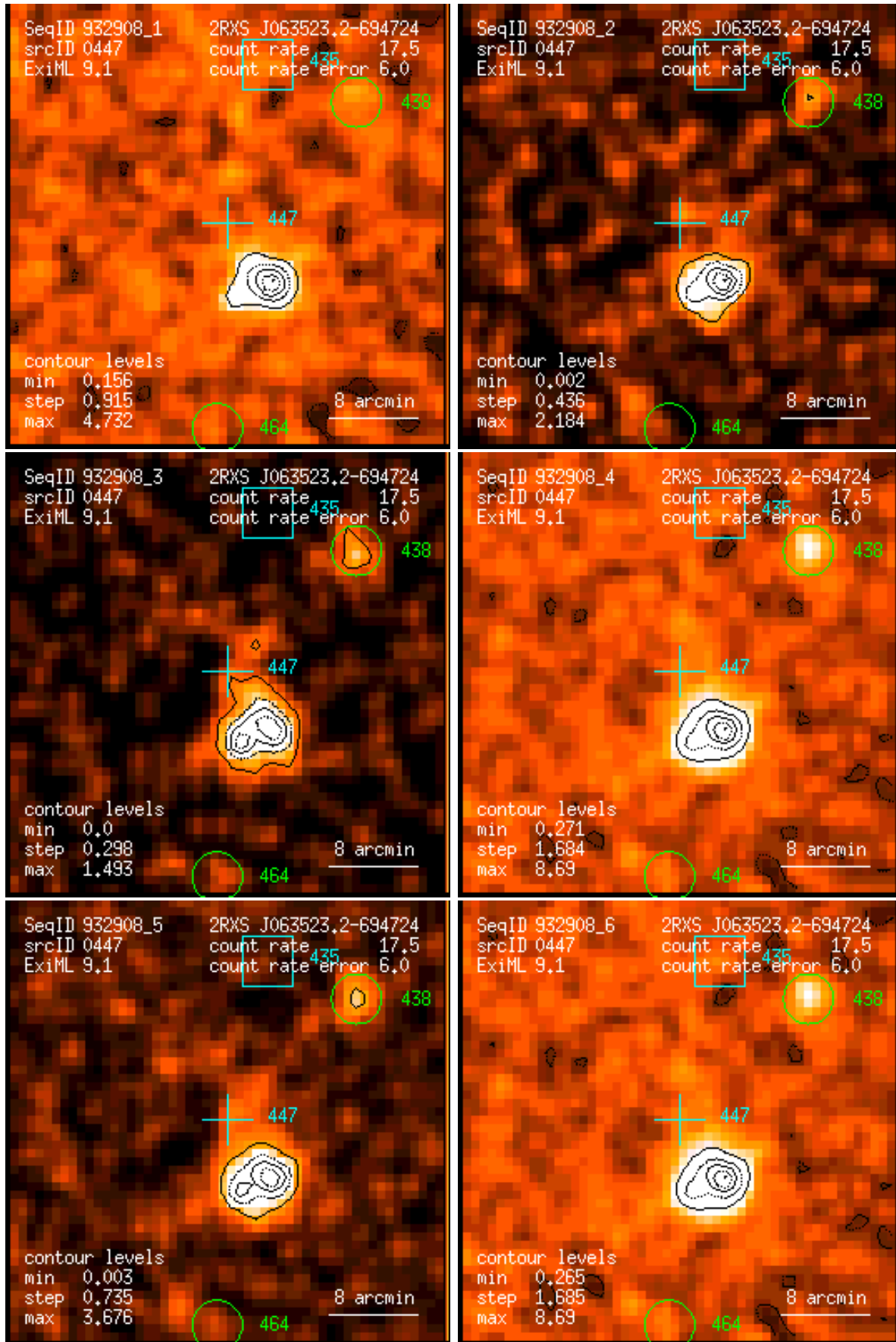
Figure 447: RASS 932908: detection 0447: band rate images, Gaussian filter: (1) PSPC channels 11 – 41, (2) 52 – 90, (3) 91 – 201, (4) 11 – 235, (5) 52 – 201, (6) 11 – 201. Broad band rates in counts/ks. Band rate contour levels in counts/ks/arcmin 2 .
